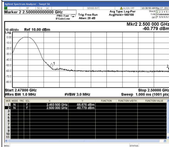
Channel 78 / 2480 MHz -Peak
