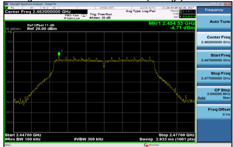
802.11g PSD FOR BANDEDGE LIMIT (CH-High)
