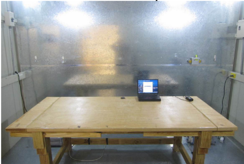
Conducted Emission Set up Photo
