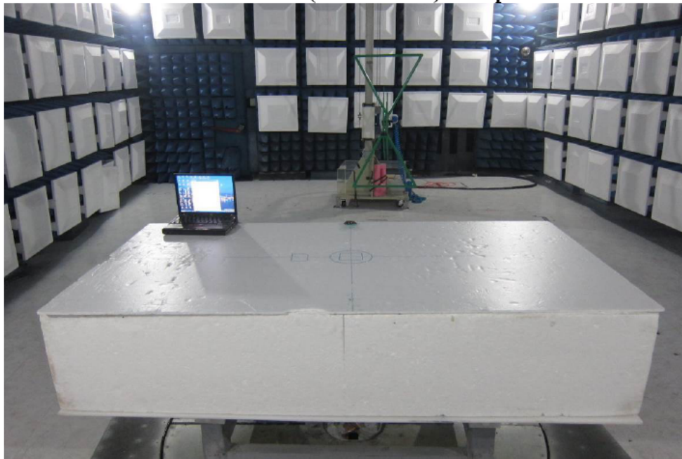
Radiated Emission (below 1GHz) Set up Photo
