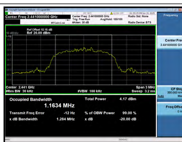
Bluetooth 3DH5 2441MHz
