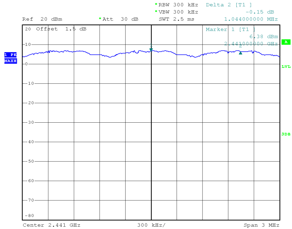
8-DPSK Mode
