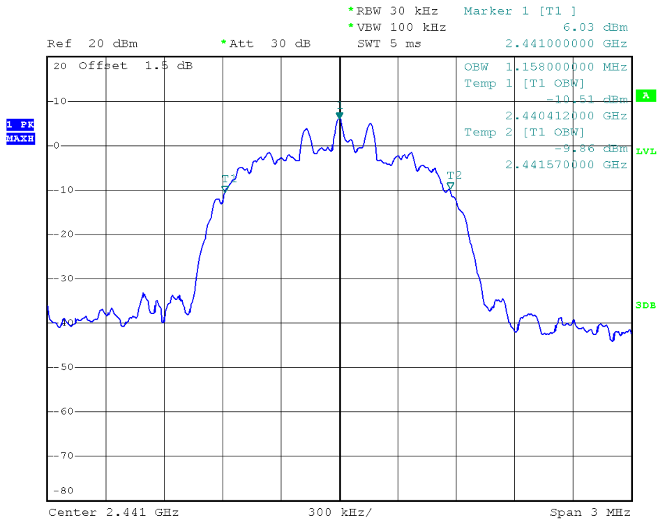
39 Channel @ 8-DPSK
