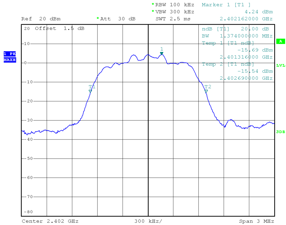
0 Channel @ 8-DPSK
