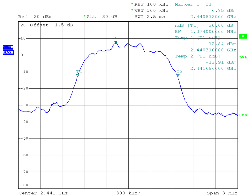
39 Channel @ 8-DPSK
