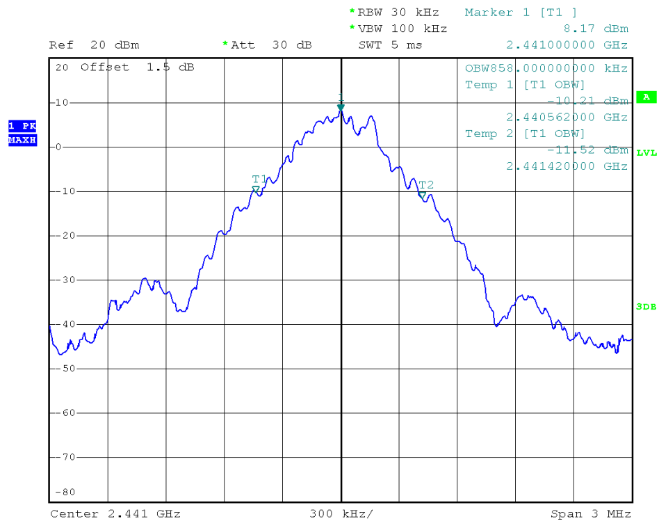
39 Channel @ GFSK
