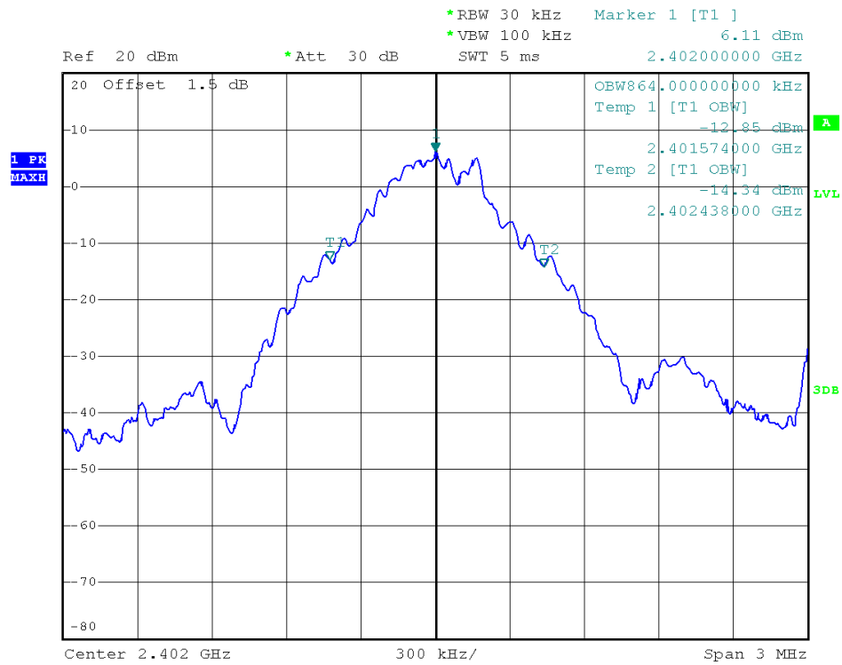
0 Channel @ GFSK
