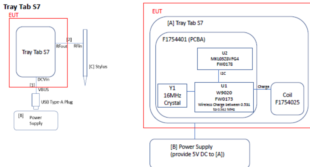
Figure 8: Block Diagram of Test Configuration
