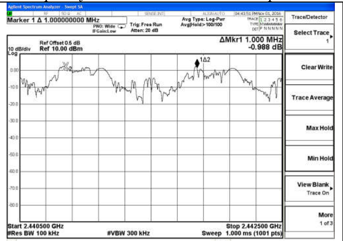
Test Plot Of Frequency Separation (2Mbps)
