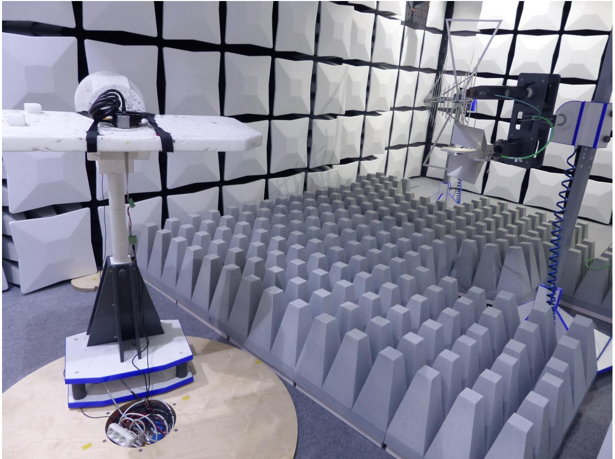
Photo 6: Test setup for radiated measurements (Enclosure, fully-anechoic chamber)
