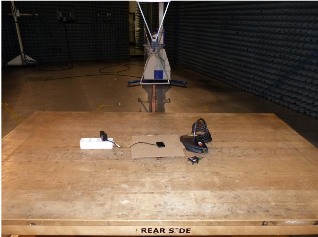
Photo 2: Test setup AB01 for radiated measurements, unintentional radiator §15) single device setup.
