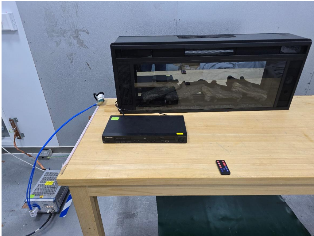
Conducted Emission
