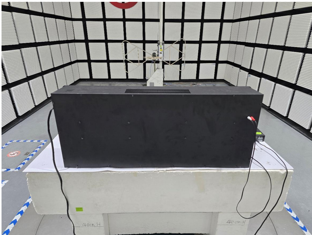
Radiated Disturbance below 1 GHz and above 30 MHz
