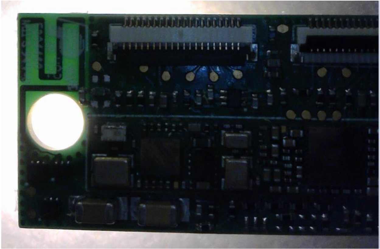
5:Delta Zulu control box lower PCBA "internal" side, antenna highlighted by backlight
