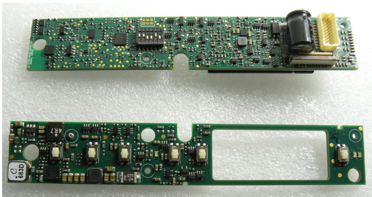
2:Delta Zulu control box upper and lower PCBA's, "external" side
