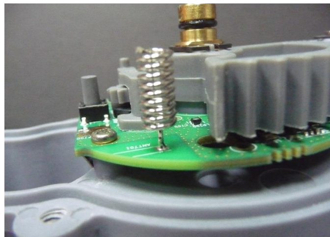
Photograph 7.6.1 Antenna assembly
