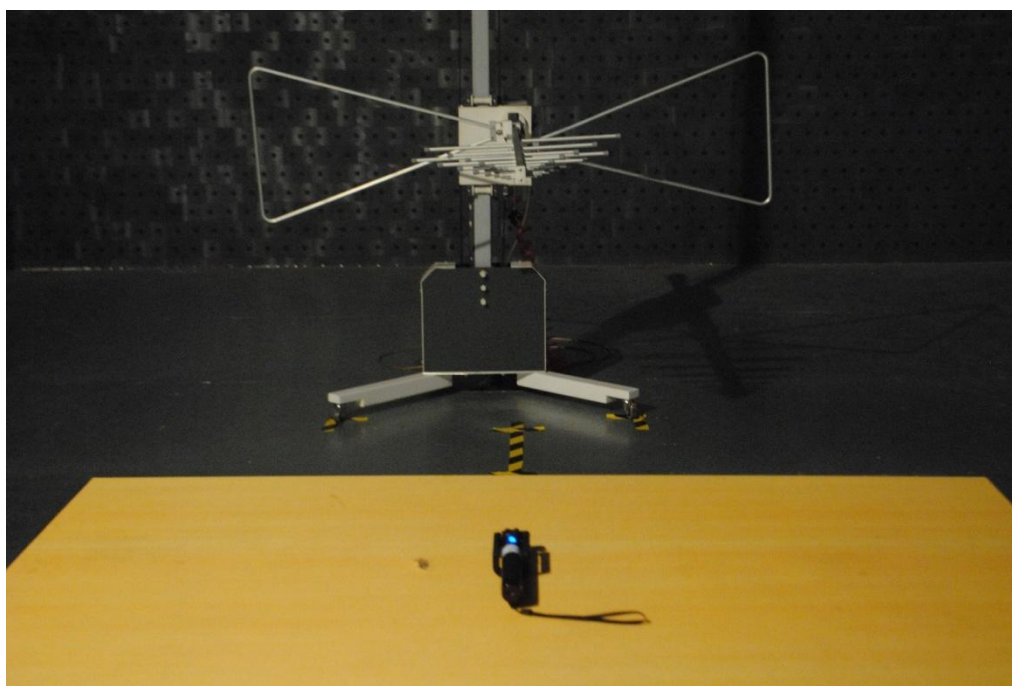
Radiated Emission test view
