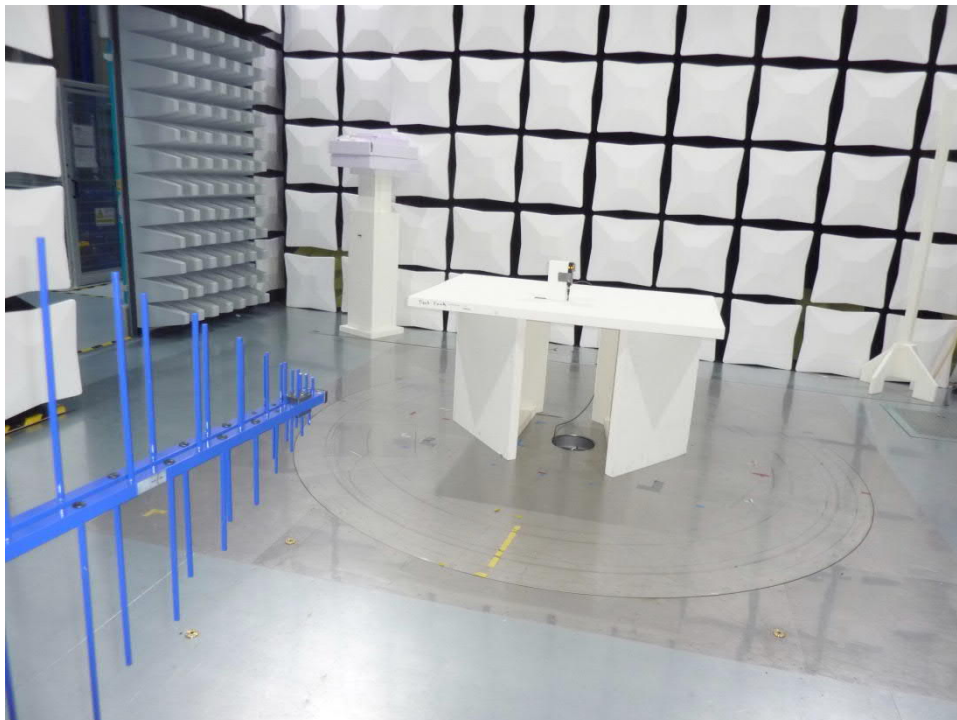
210165_06: Test setup radiated emission test 30 – 1000 MHz
