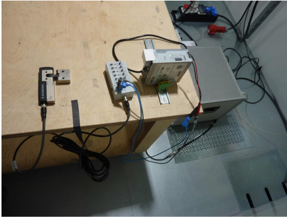
210165_01: Test setup conducted emission test 150 kHz – 30 MHz
