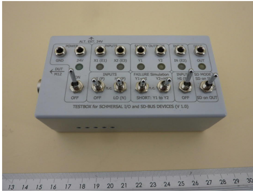
210165_EUT13: Testbox view
