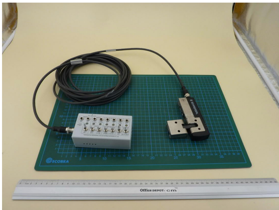
210165_EUT12: Setup view
