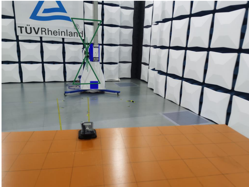
Photographs 1-2: Set-up for Field strength of fundamental and Unwanted Emissions in the Spurious Domain
