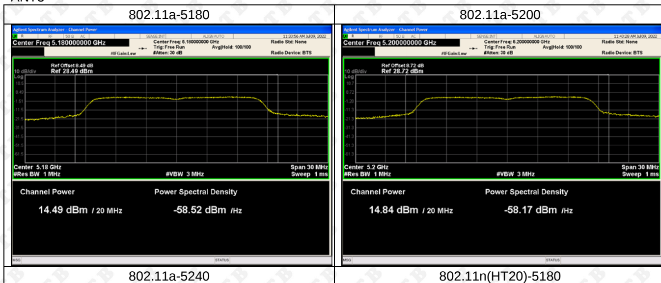
802.11a-5180
