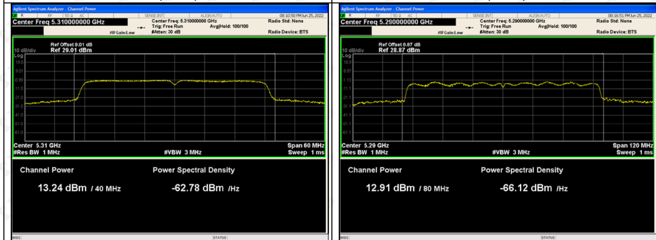
802.11ac(VH40)-5310
