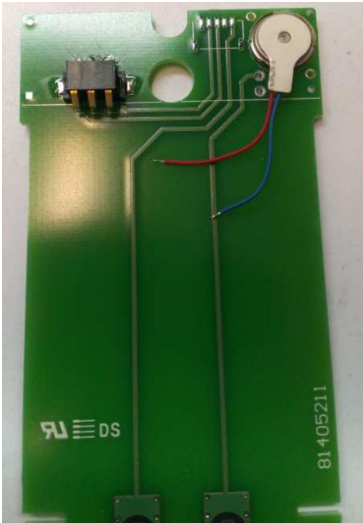
Backside PCB – front
