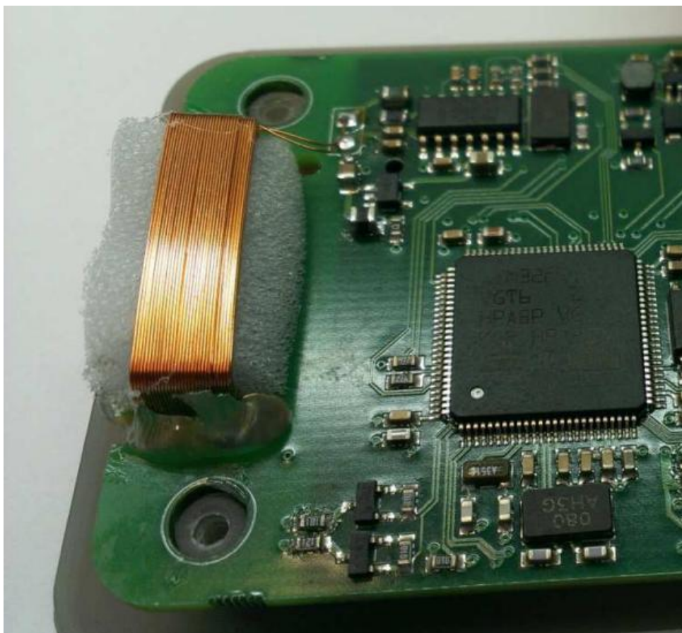
RFID antenna assembly
