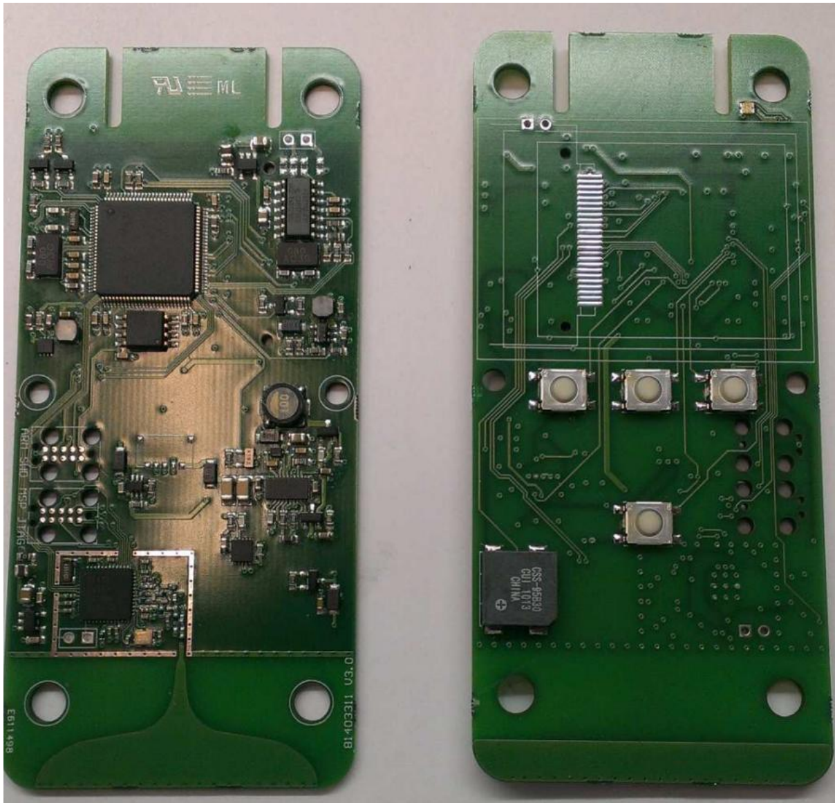
Frontside PCB, inner side (left) and Reader front side (right)
