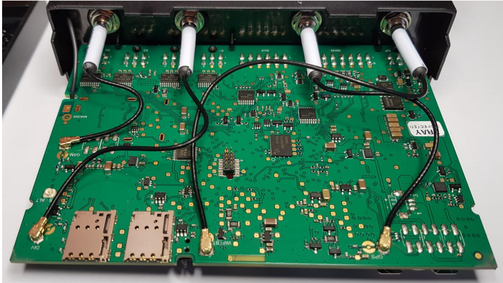
Figure 7: Bottom view to show routing of RF pigtailed
