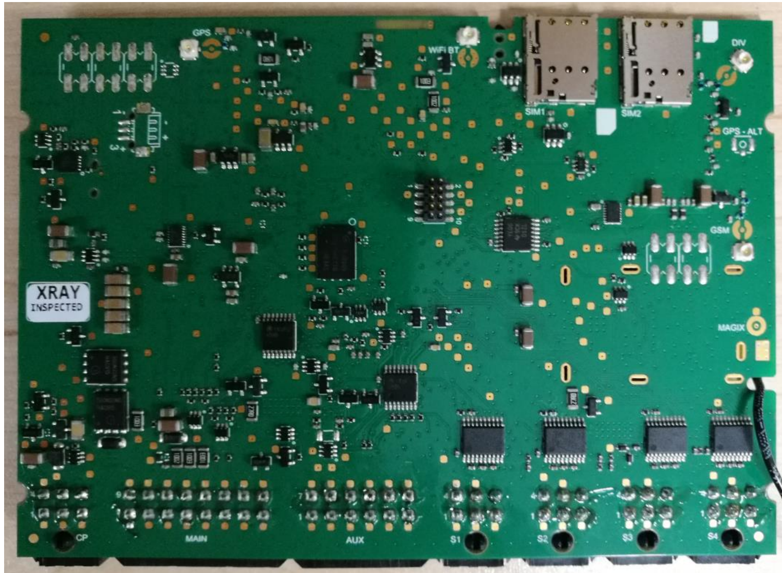
Figure 2: Bottom Side of PCB
