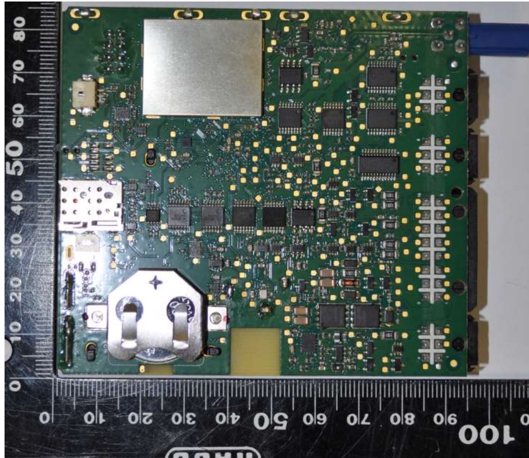
Figure 8: Bottom Side of PCB
