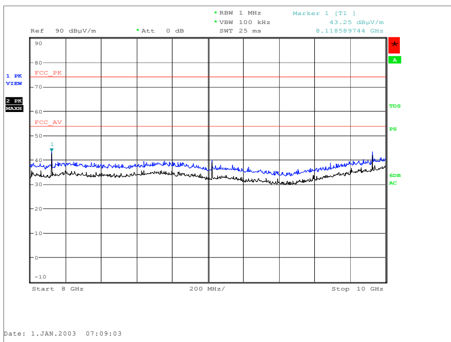
Figure 16 - 902.2 MHz - 8 GHz to 10 GHz - X Orientation - Horizontal and Vertical
