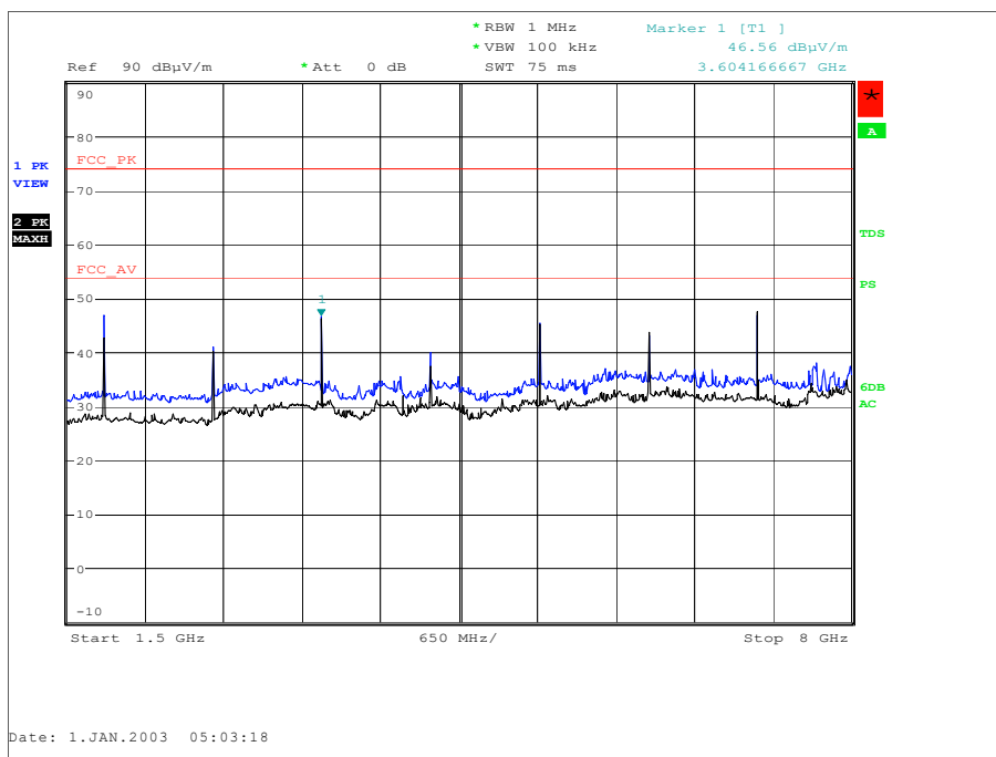
Figure 15 - 902.2 MHz - 1.5 GHz to 8 GHz - X Orientation - Horizontal and Vertical
