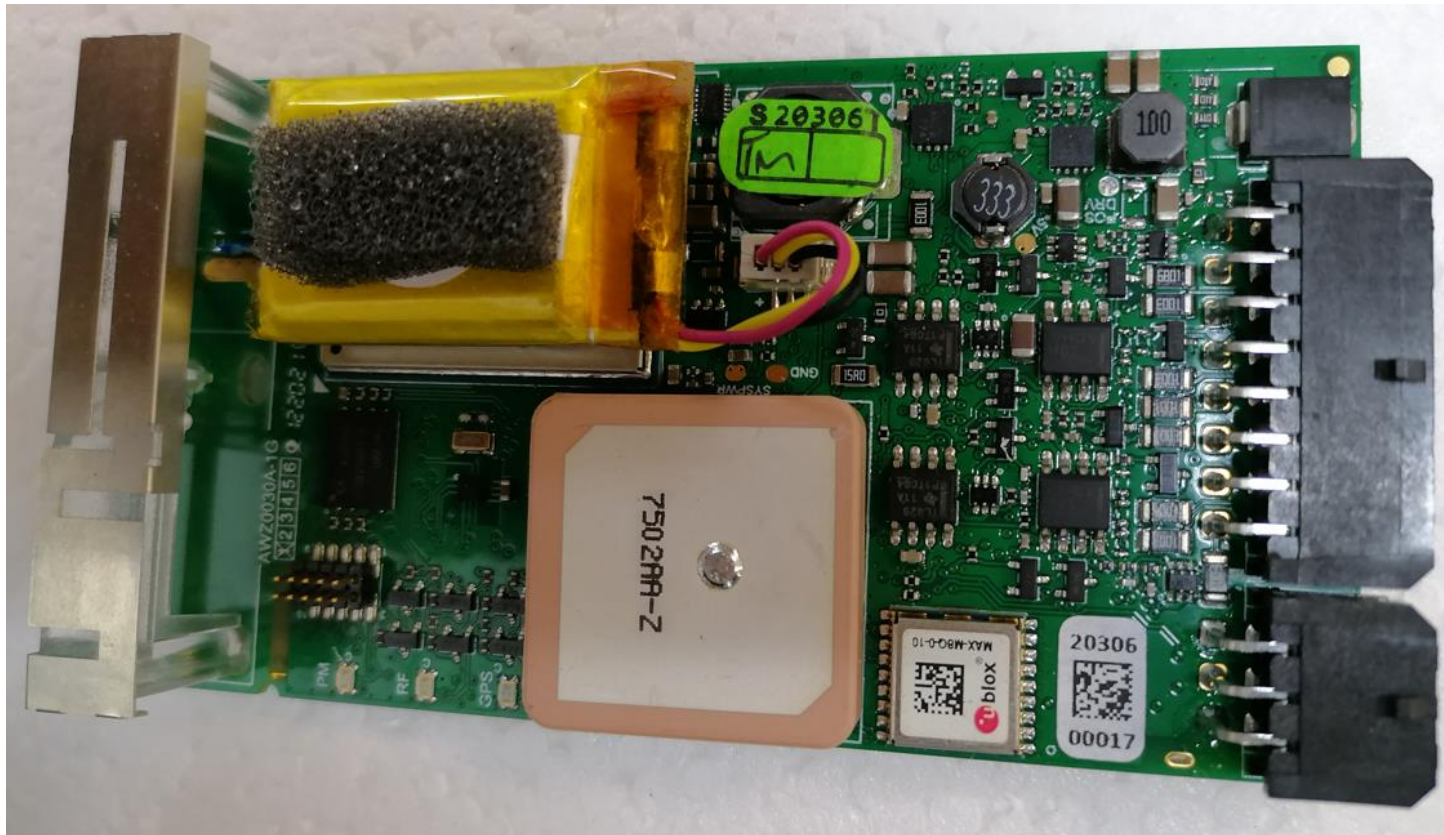
Figure 2: PCB top view, with battery fitted
