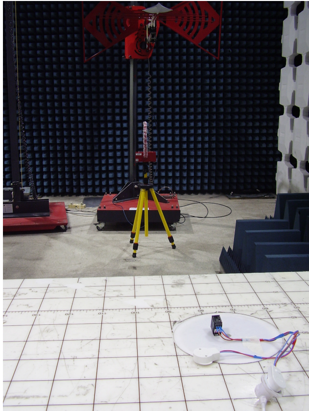
Photo 3. RE test setup
