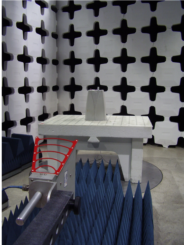
Photo 1. RE test setup
