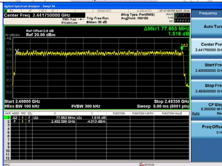
8DPSK Modulation
