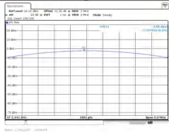
Peak Output Power \pi/4 QPSK_Channel 39
