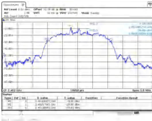
8DPSK_3-DH5_Channel 0
