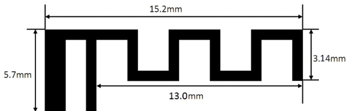
Antenna Photo &amp; Length (mm)
