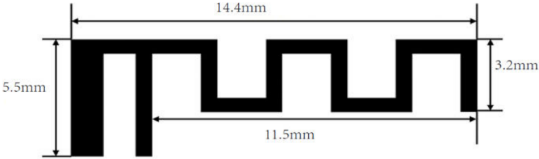
Antenna Photo & Length (mm)
