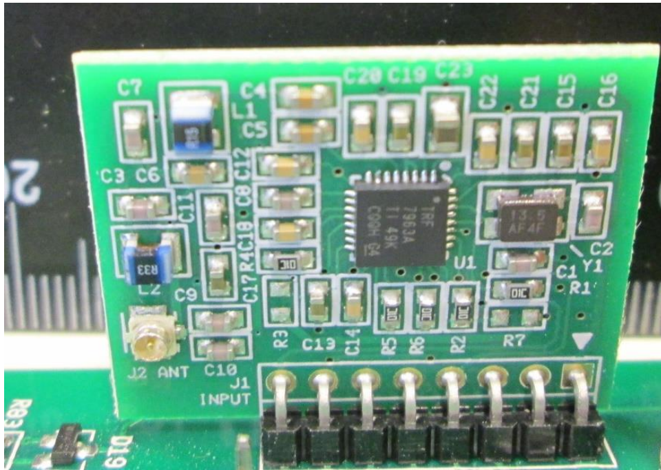
RFID board, close-up – View 1
