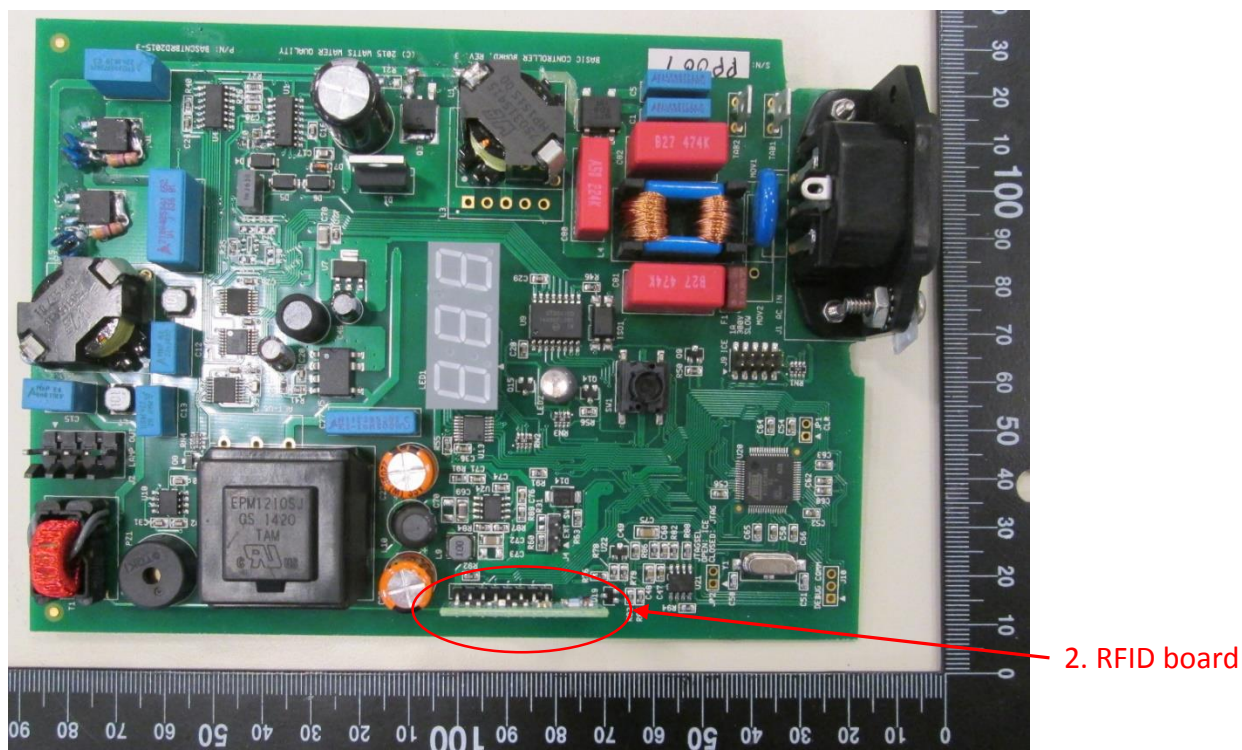
Controller main PCB – View 1
