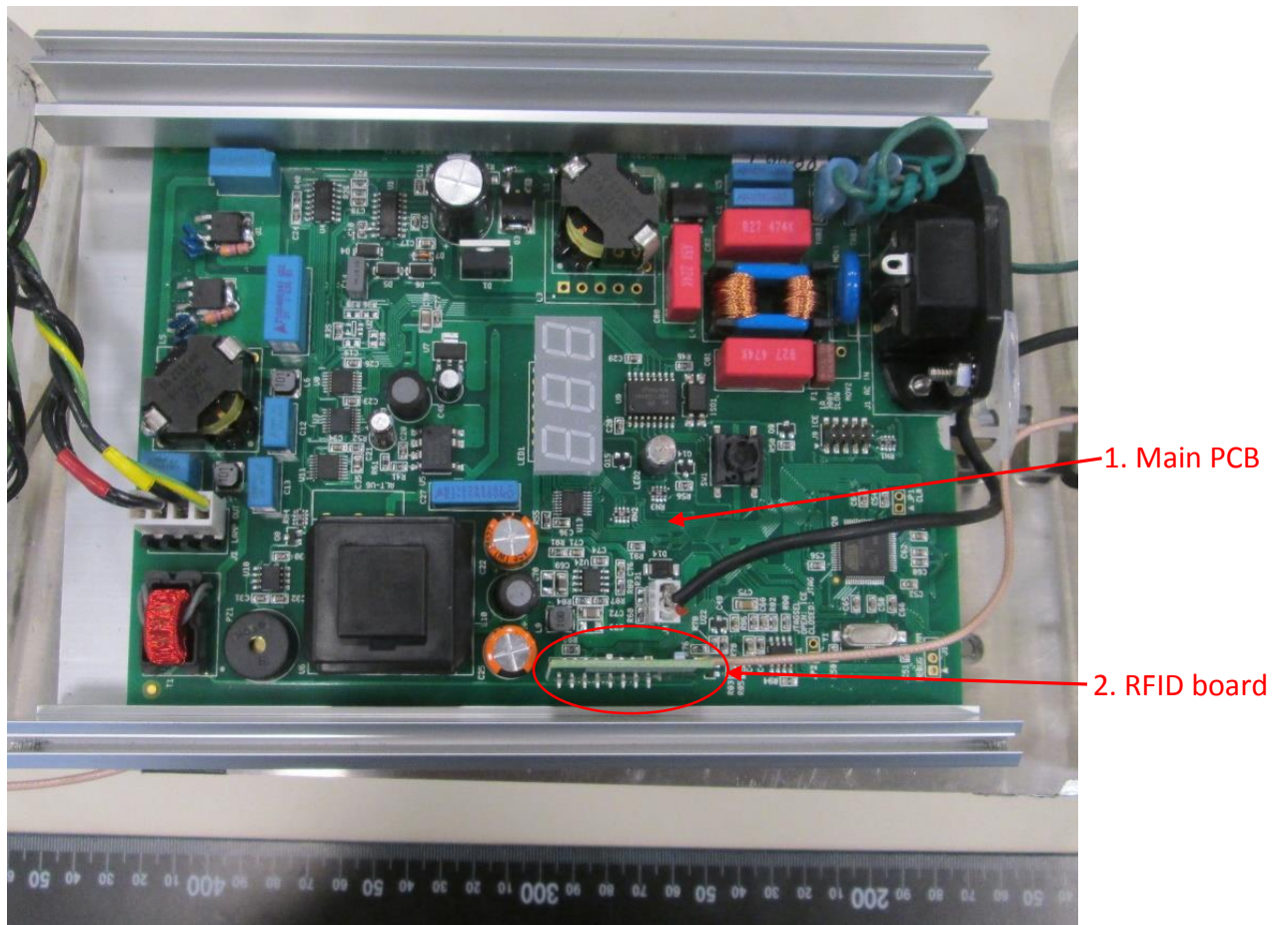
Controller enclosure opened
