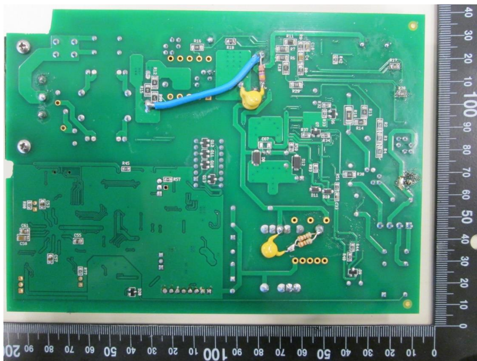
Controller main PCB – View 2
