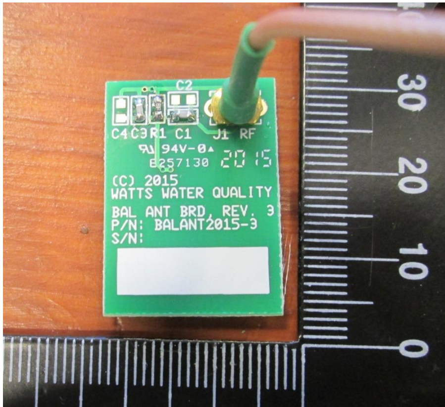
RFID antenna – View 1
