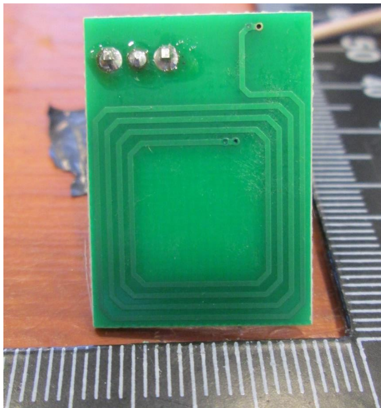
RFID antenna – View 2
