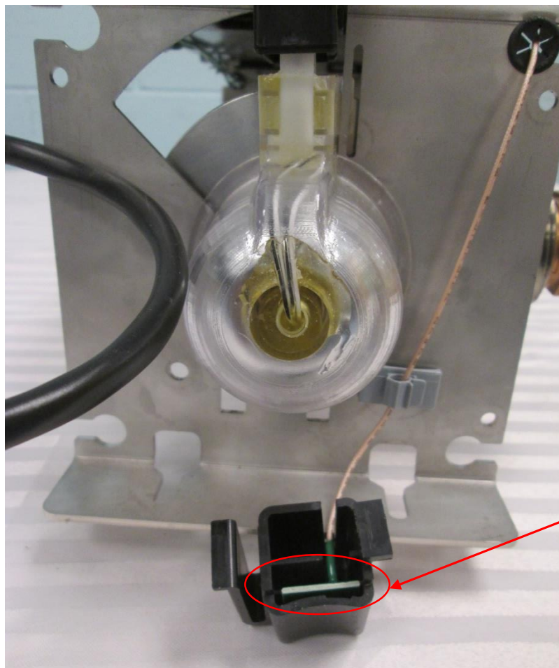
RFID antenna, cover opened
