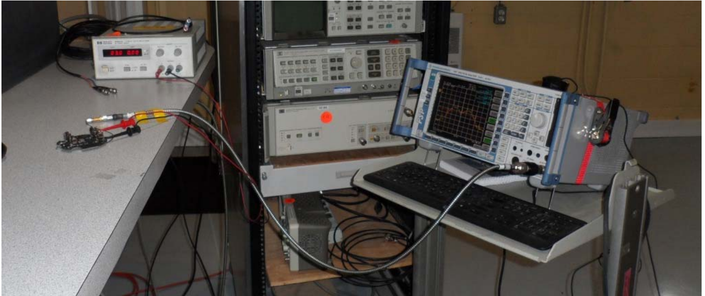
Figure E21.1 – Setup Photo – Conducted Measurements
