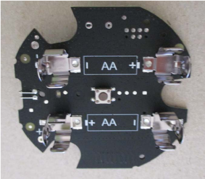
Figure E20.2 – Internal Photo – PCB Top View
