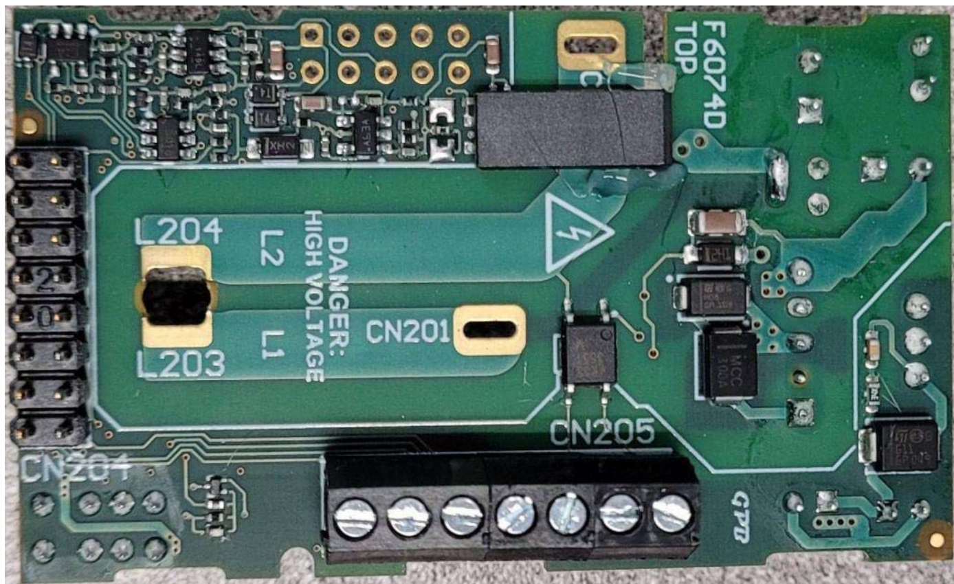
Figure E22.4 – F6074D – Top View
