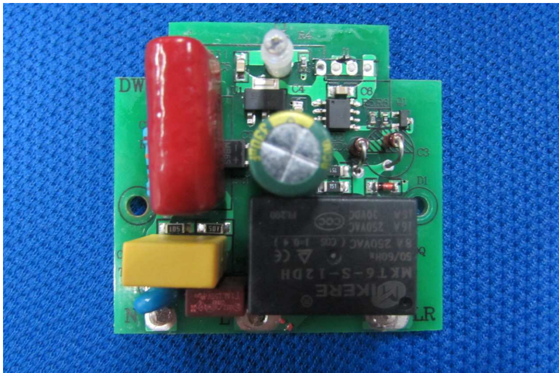
PCB View remove RF receiver module
