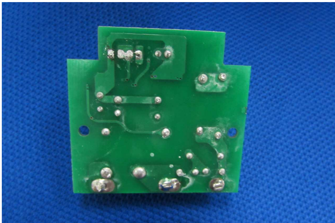
PCB Other side
