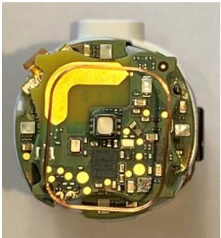
Figure 1: PCB Front
