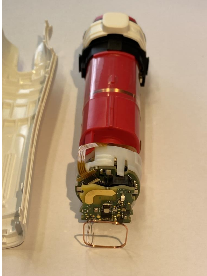
Figure 5: Assembled View
