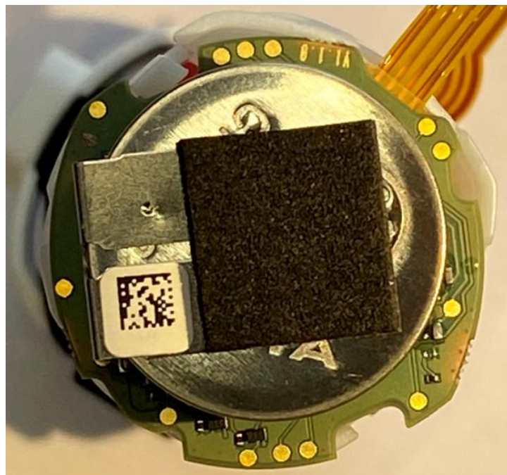
Figure 4: PCB Bottom
