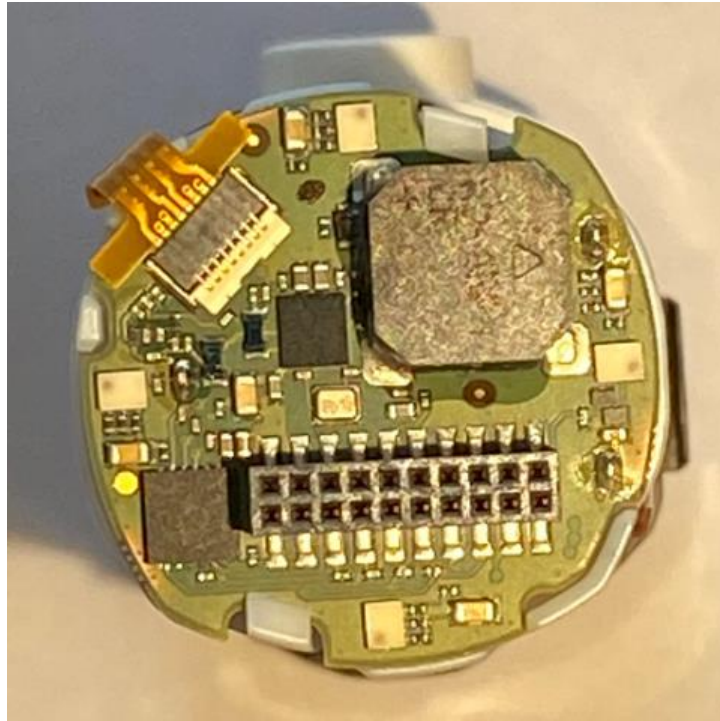
Figure 3: PCB Front
