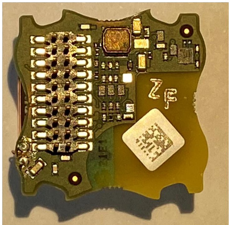
Figure 2: PCB Bottom
