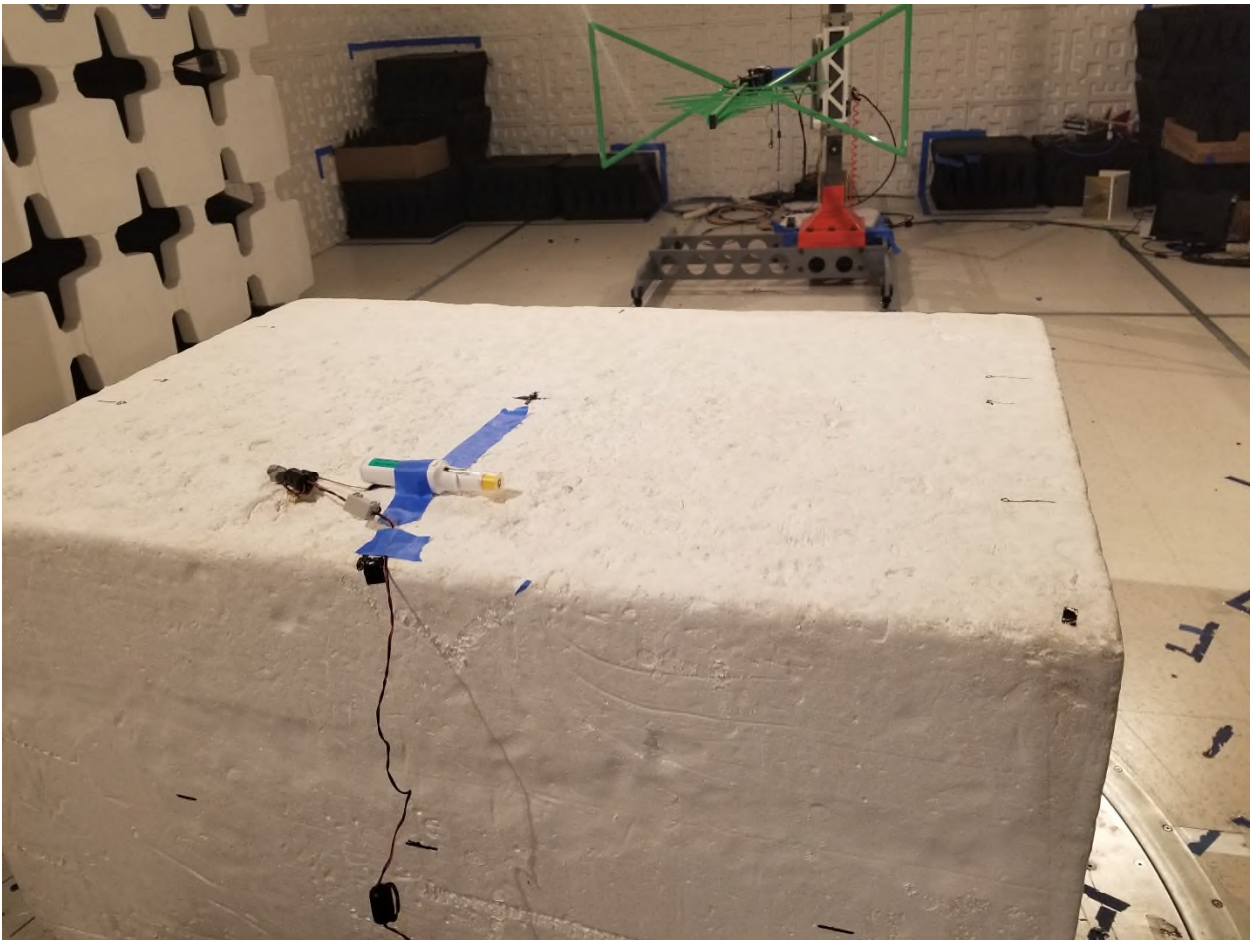
Figure 4: Radiated Emissions – Rear View
