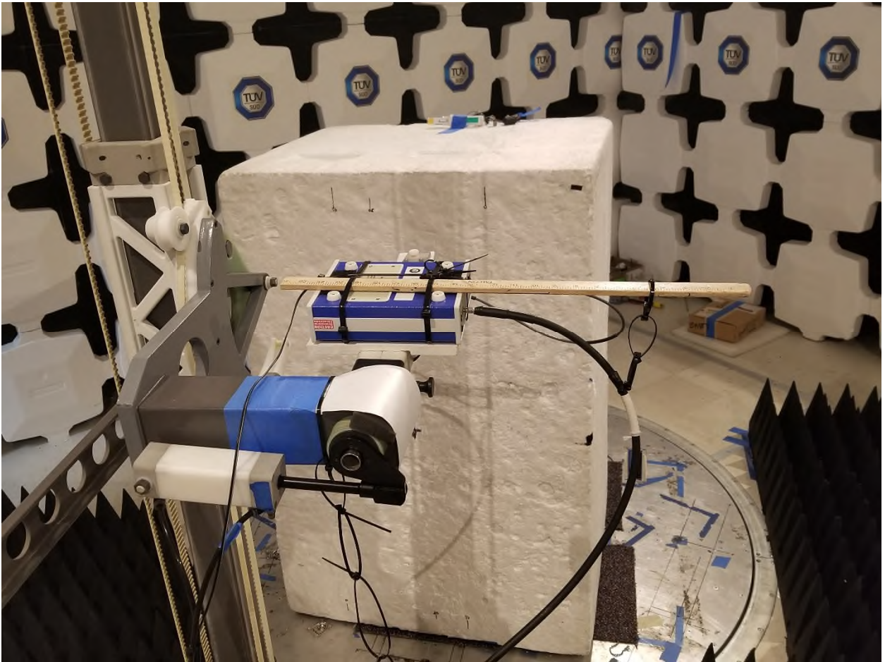
Figure 7: Radiated Emissions – Front View
