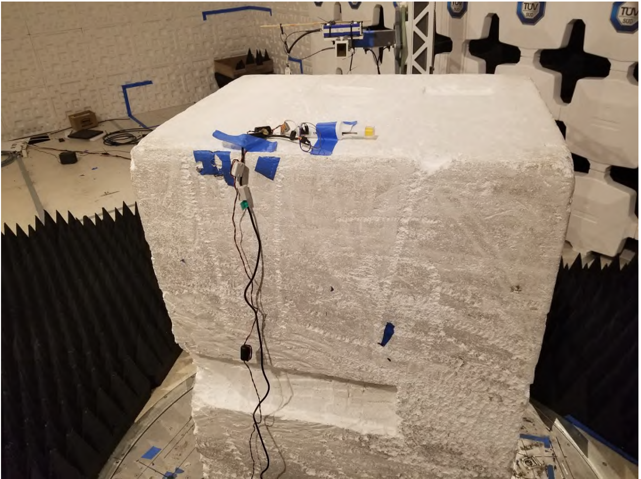
Figure 8: Radiated Emissions – Back View
