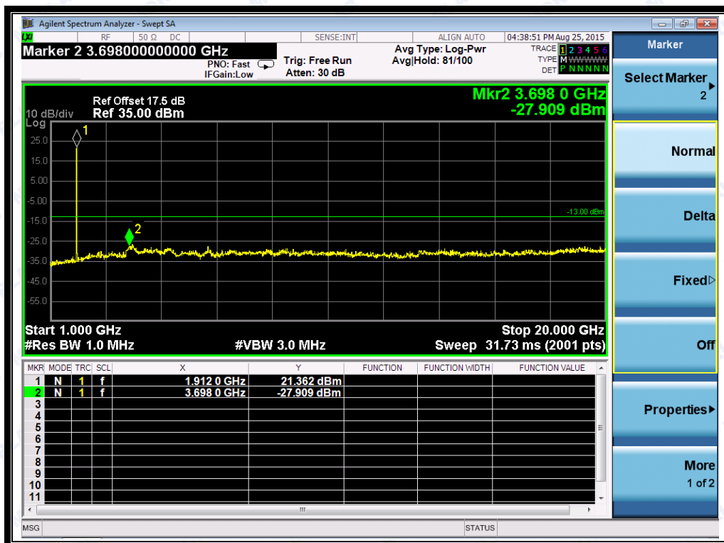
(Plot I3.1: WCDMA1900MHz Channel = 9538 1GHz to 20GHz)
