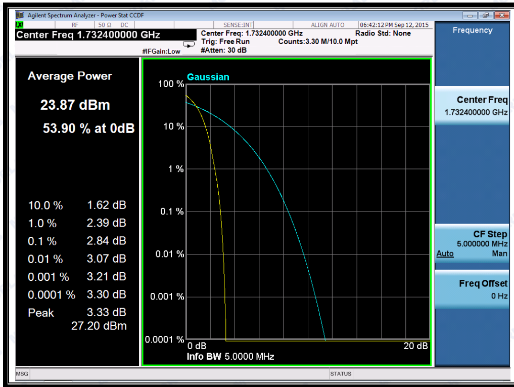
(Plot D2: WCDMA 1700MHz Channel = 1412)
