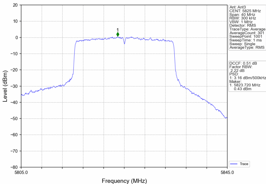
802.11ax(HEW20)_HCH_5825MHz_RU242_Left_Ant3_NTNV
