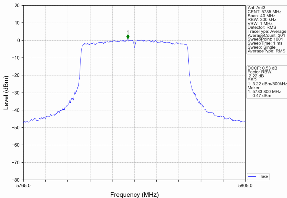
802.11ax(HEW20)_MCH_5785MHz_RU242_Left_Ant3_NTNV
