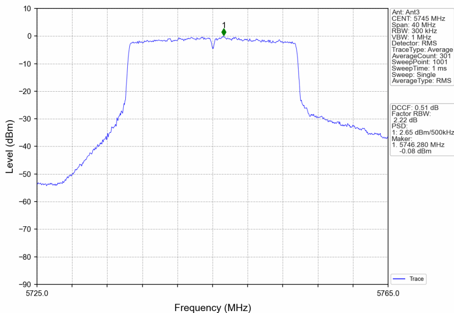
802.11ax(HEW20)_LCH_5745MHz_RU242_Left_Ant3_NTNV
