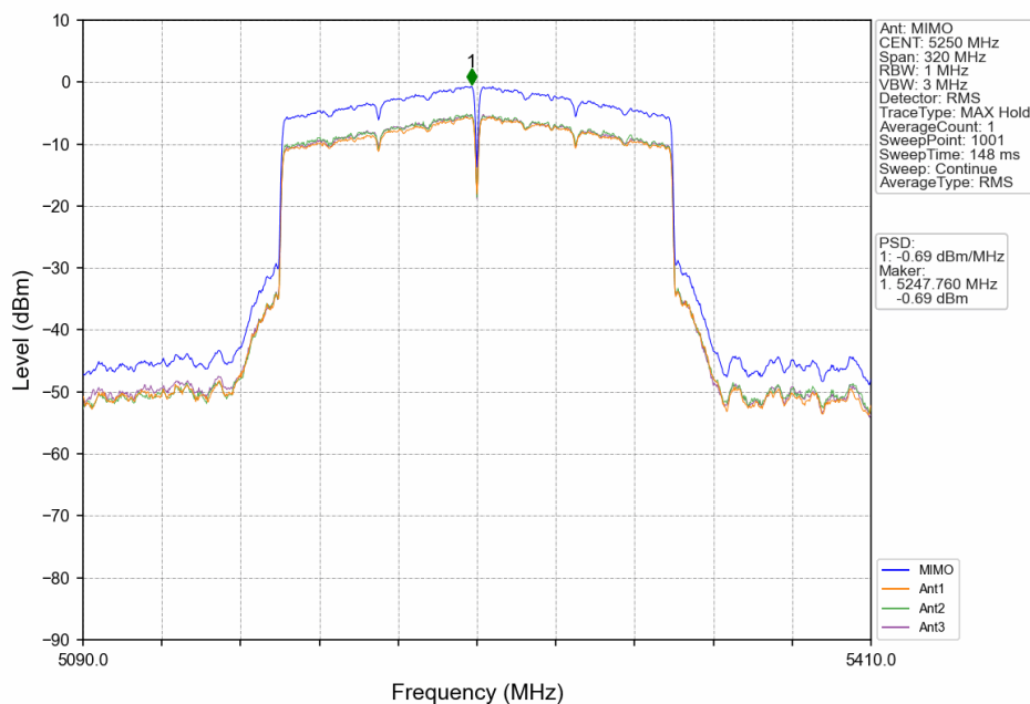
802.11ax(HEW160)_MCH_5250MHz_2xRU996_Left_MIMO_NTNV
