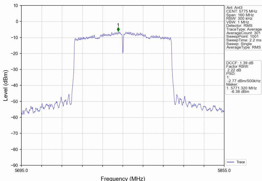
802.11ac(VHT80)_MCH_5775MHz_Ant3_NTNV
