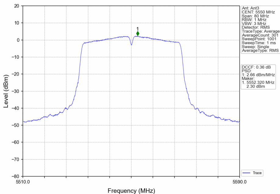
802.11n(HT40)_MCH_5550MHz_Ant3_NTNV
