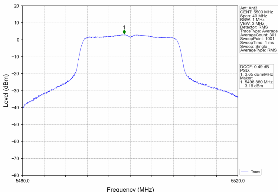
802.11ac(VHT20)_LCH_5500MHz_Ant3_NTNV
