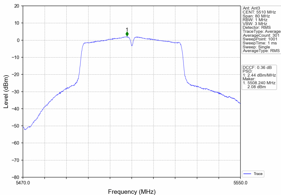
802.11n(HT40)_LCH_5510MHz_Ant3_NTNV
