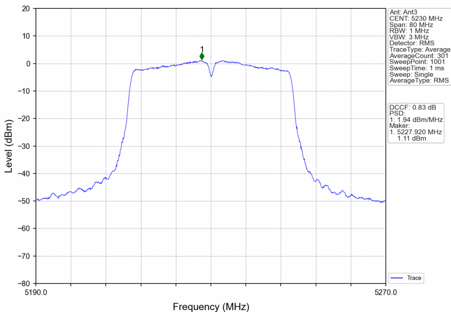
802.11ac(VHT40)_HCH_5230MHz_Ant3_NTNV
