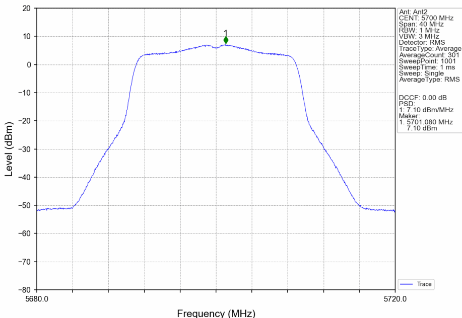
802.11n(HT20)_HCH_5700MHz_MIMO_NTNV
