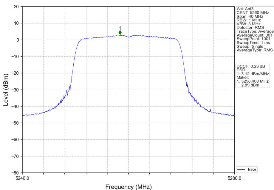
802.11ax(HEW20)_LCH_5260MHz_RU242_Left_Ant3_NTNV
