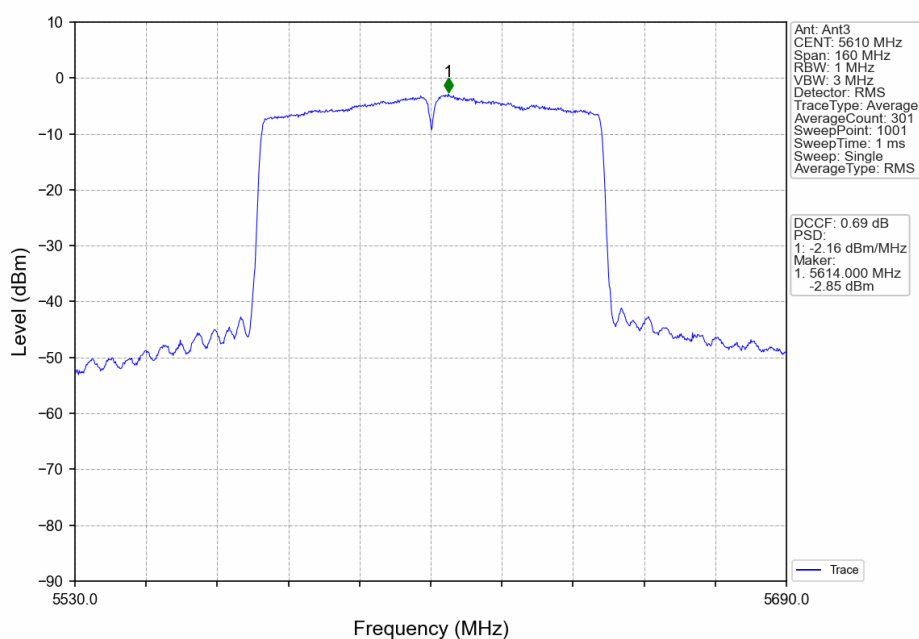
802.11ac(VHT80)_HCH_5610MHz_Ant3_NTNV
