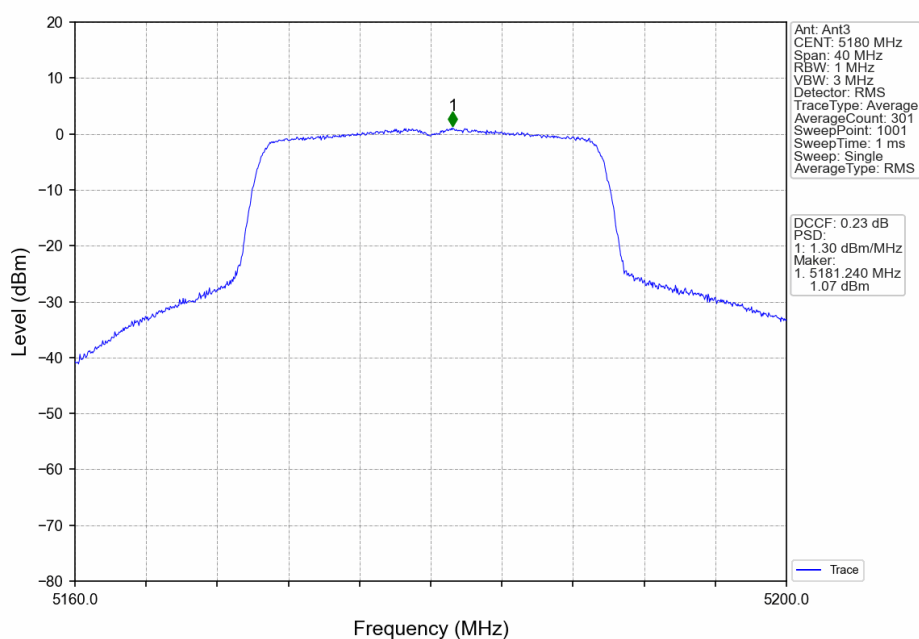
802.11ax(HEW20)_LCH_5180MHz_RU242_Left_Ant3_NTNV
