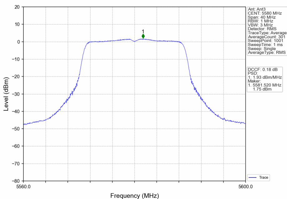
802.11ac(VHT20)_MCH_5580MHz_Ant3_NTNV
