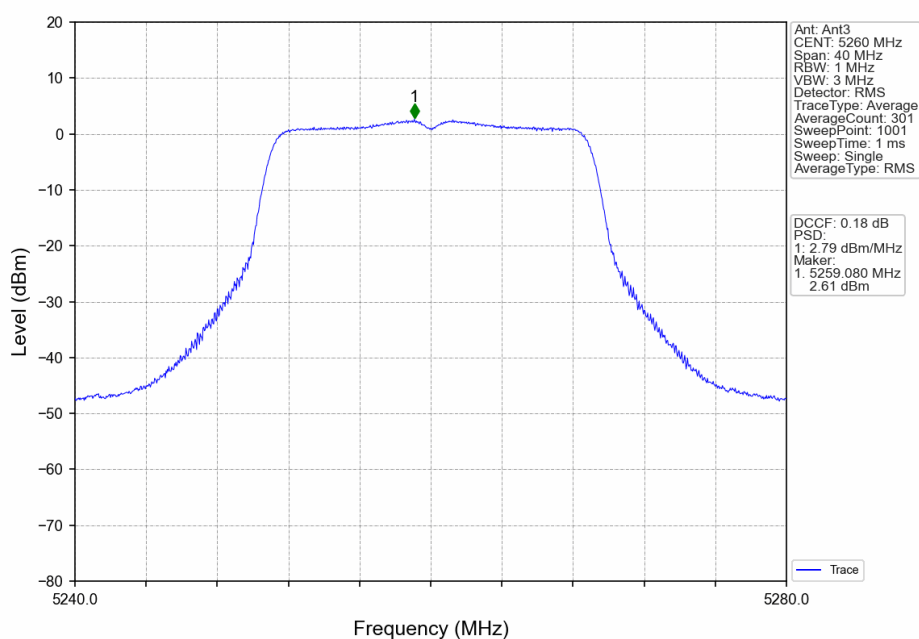
802.11ac(VHT20)_LCH_5260MHz_Ant3_NTNV
