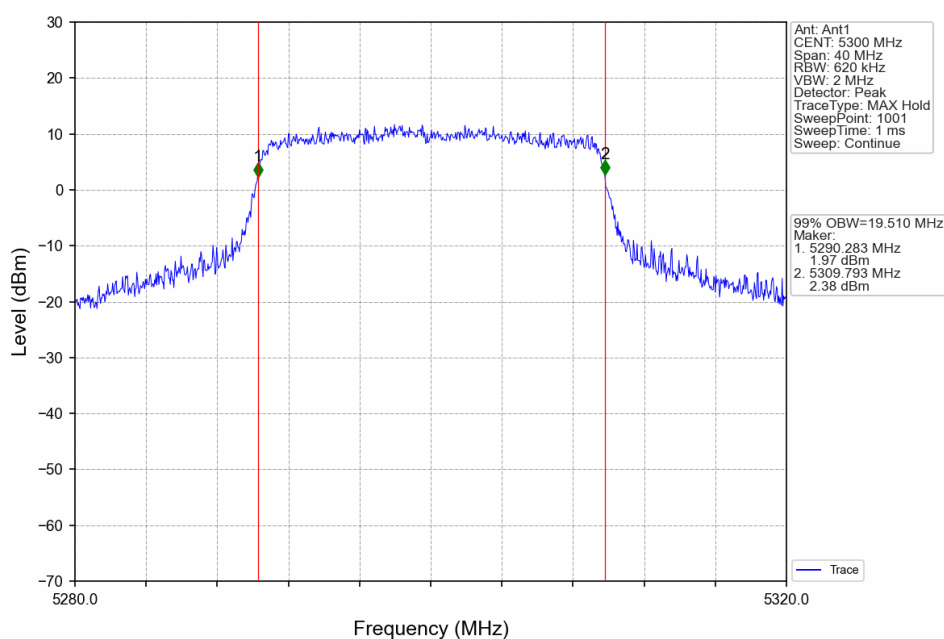
802.11ax(HEW20)_MCH_5300MHz_RU242_Left_Ant1_NTNV
