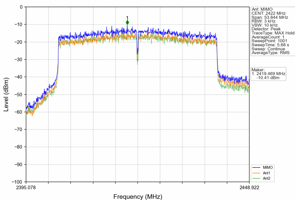
802.11ax(HEW40)_LCH_2422MHz_RU484_Left_MIMO_NTNV
