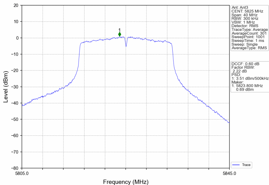
802.11ac(VHT20)_HCH_5825MHz_Ant3_NTNV
