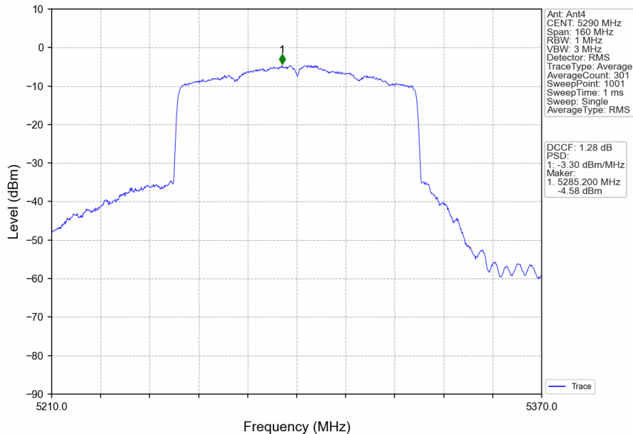
802.11ax(HEW80)_MCH_5290MHz_RU996_Left_MIMO_NTNV
