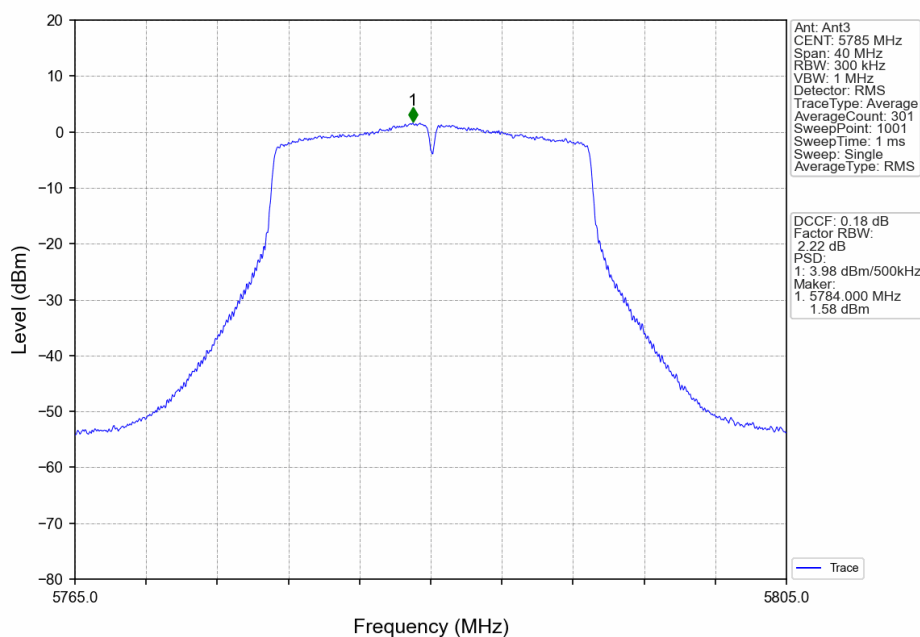
802.11n(HT20)_MCH_5785MHz_Ant3_NTNV
