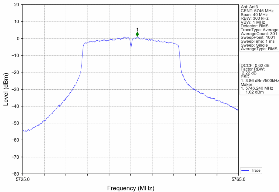
802.11ac(VHT20)_LCH_5745MHz_Ant3_NTNV
