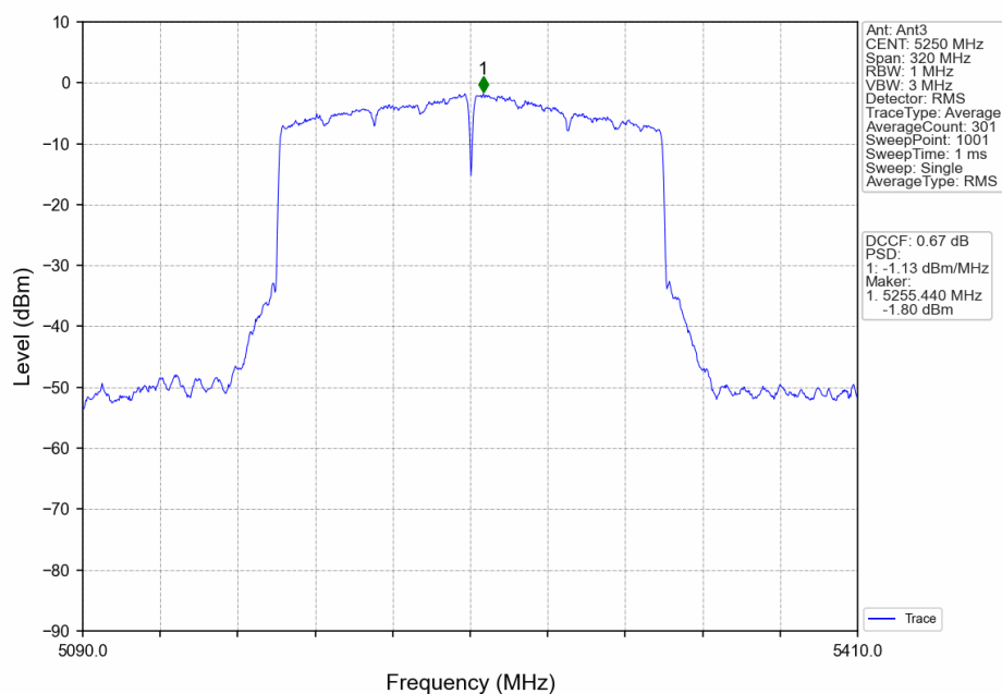
802.11ax(HEW160)_MCH_5250MHz_2xRU996_Left_Ant3_NTNV
