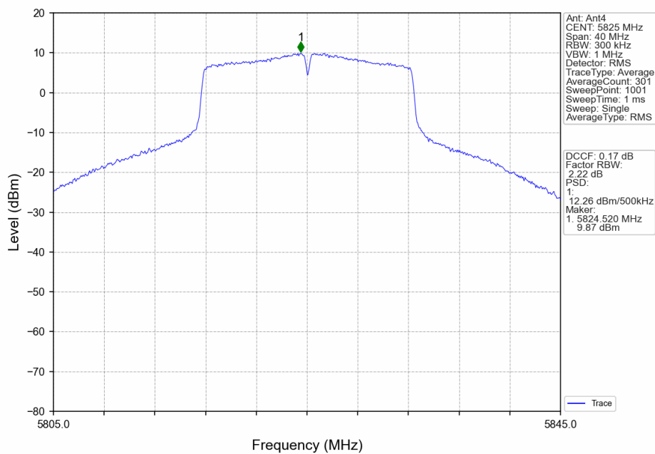
802.11a_HCH_5825MHz_Ant4_NTNV
