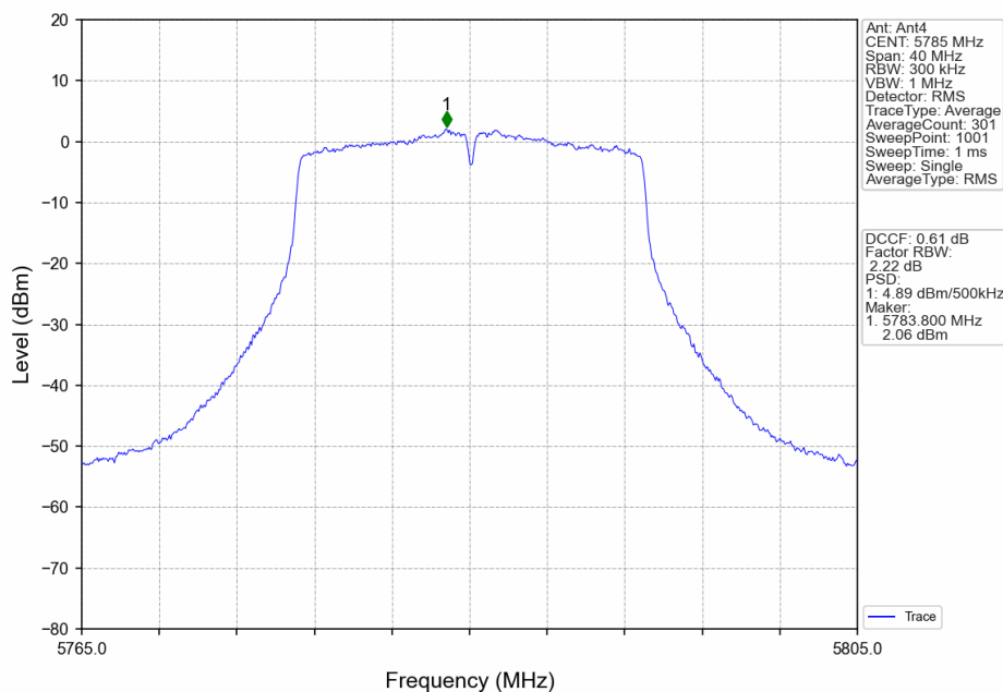
802.11ac(VHT20)_MCH_5785MHz_Ant4_NTNV
