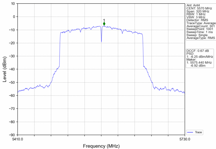
802.11ax(HEW160)_MCH_5570MHz_2xRU996_Left_Ant4_NTNV
