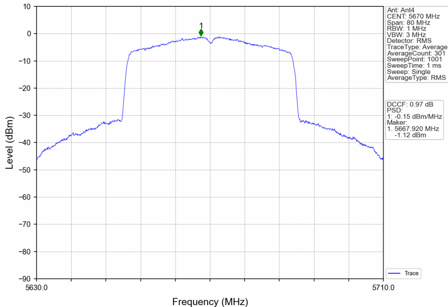
802.11ax(HEW40)_HCH_5670MHz_RU484_Left_MIMO_NTNV
