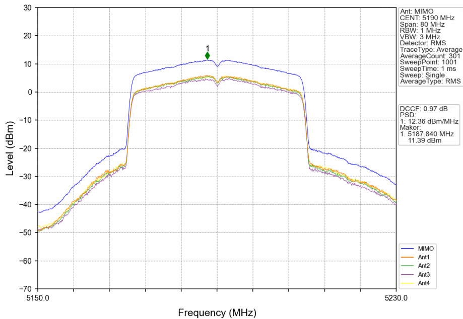
802.11ax(HEW40)_LCH_5190MHz_RU484_Left_MIMO_NTNV
