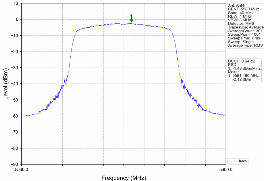
802.11ax(HEW20)_MCH_5580MHz_RU242_Left_MIMO_NTNV
