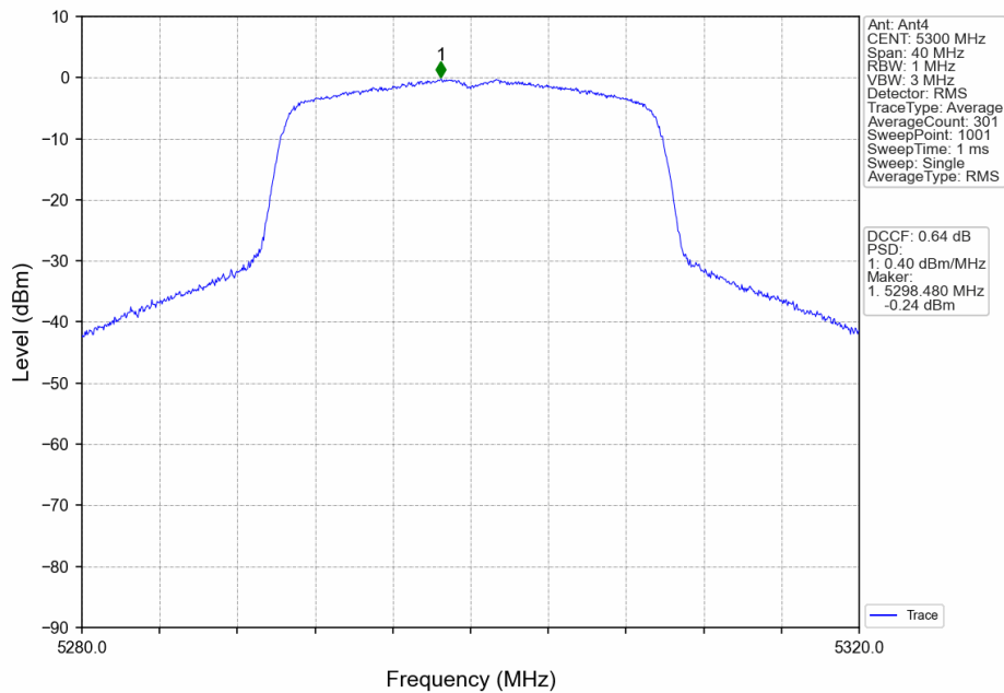
802.11ax(HEW20)_MCH_5300MHz_RU242_Left_Ant4_NTNV
