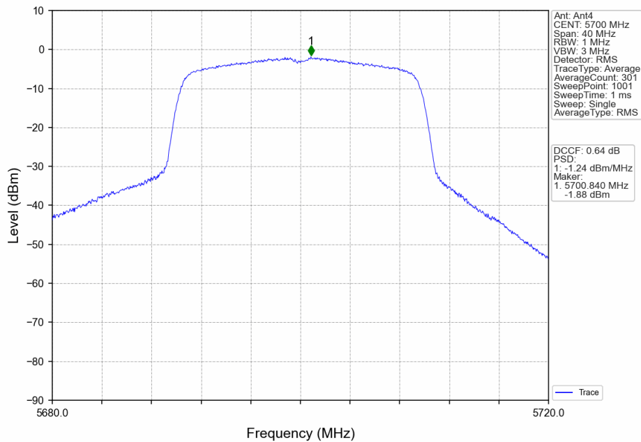
802.11ax(HEW20)_HCH_5700MHz_RU242_Left_Ant4_NTNV
