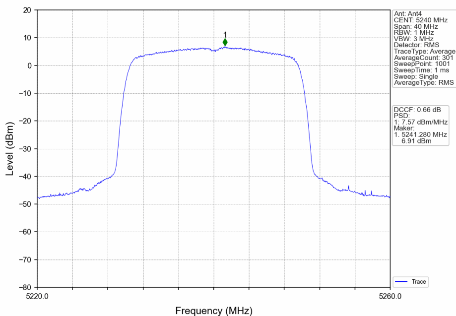
802.11ax(HEW20)_HCH_5240MHz_RU242_Left_Ant4_NTNV
