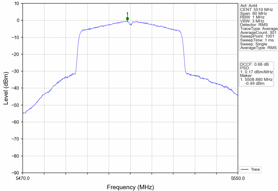
802.11ax(HEW40)_LCH_5510MHz_RU484_Left_MIMO_NTNV
