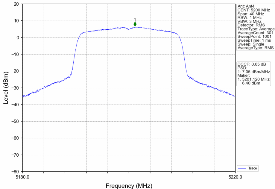
802.11ax(HEW20)_MCH_5200MHz_RU242_Left_MIMO_NTNV
