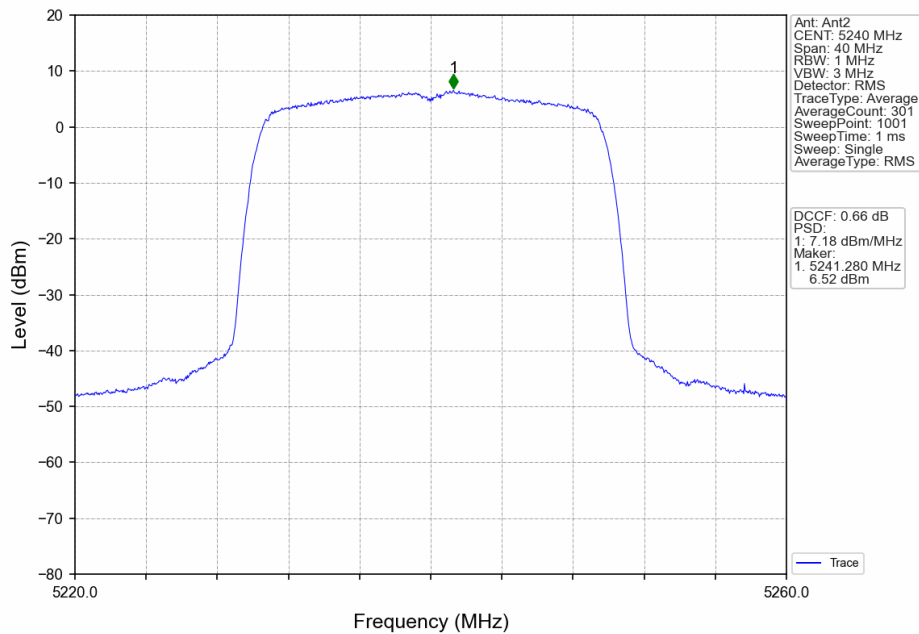
802.11ax(HEW20)_HCH_5240MHz_RU242_Left_Ant2_NTNV
