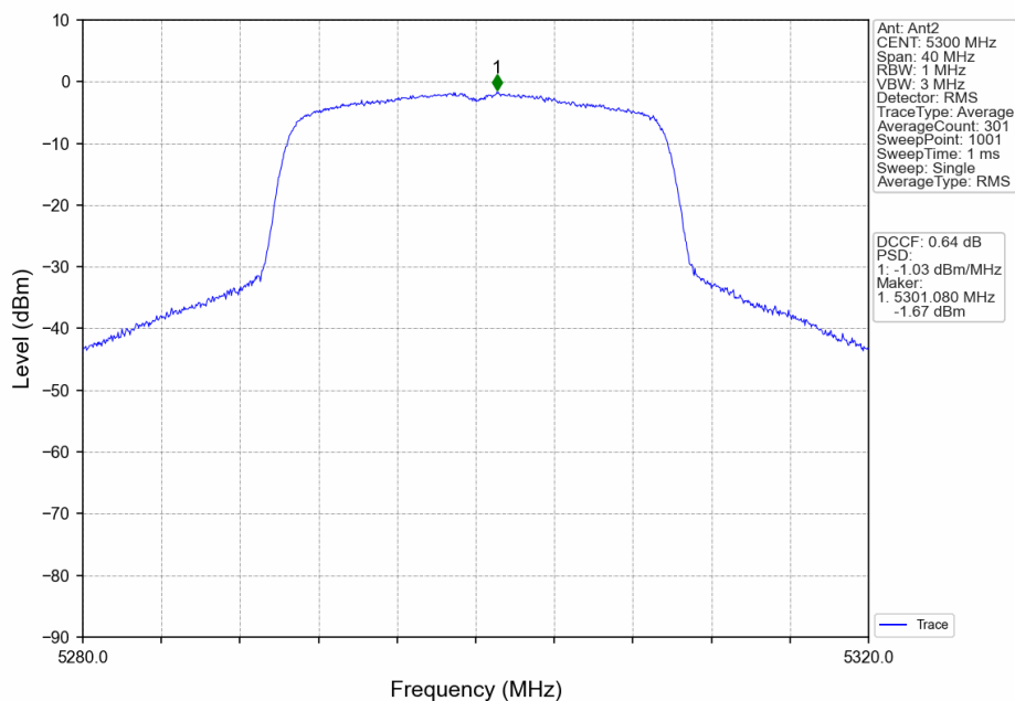
802.11ax(HEW20)_MCH_5300MHz_RU242_Left_Ant2_NTNV
