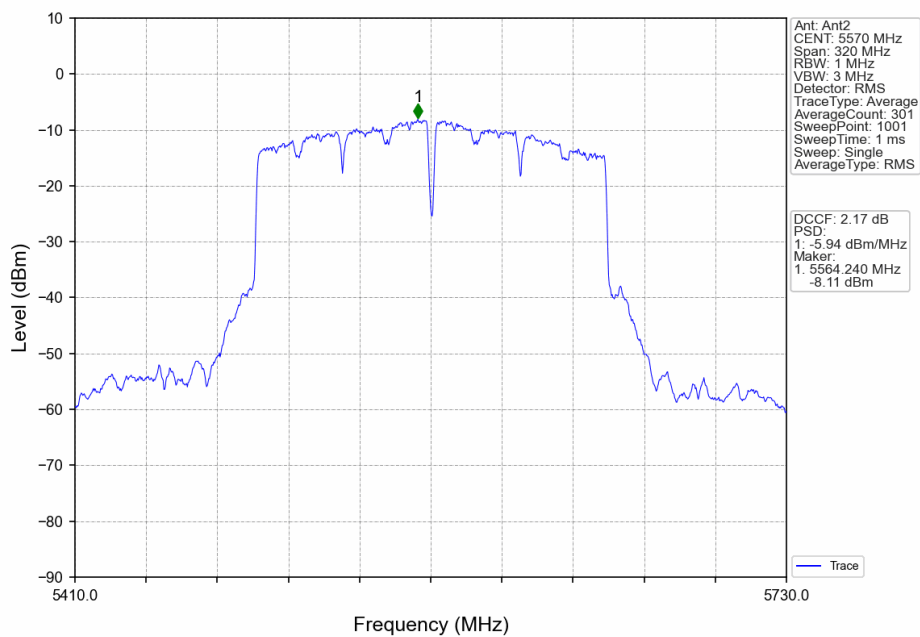
802.11ac(VHT160)_MCH_5570MHz_Ant2_NTNV
