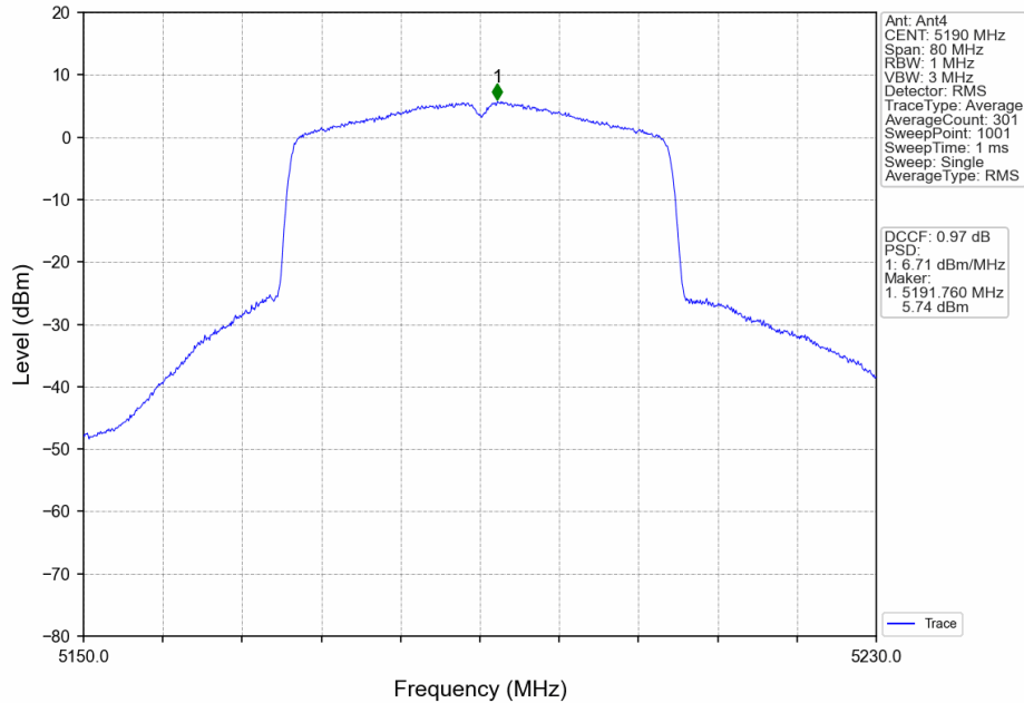
802.11ax(HEW40)_LCH_5190MHz_RU484_Left_MIMO_NTNV
