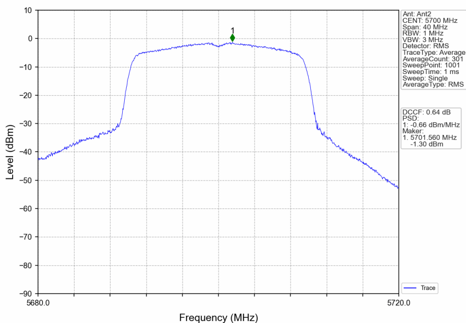
802.11ax(HEW20)_HCH_5700MHz_RU242_Left_Ant2_NTNV
