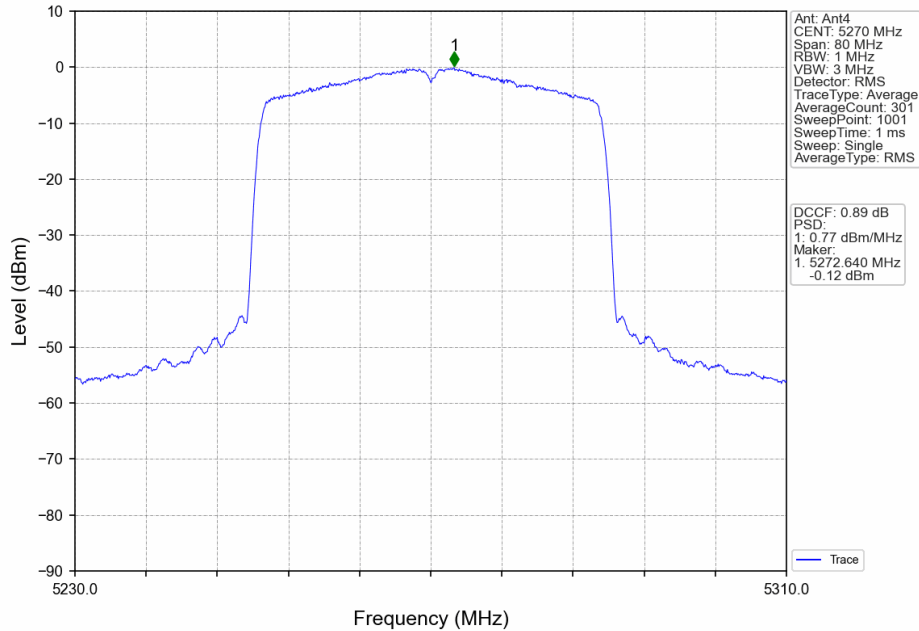
802.11ax(HEW40)_LCH_5270MHz_RU484_Left_MIMO_NTNV
