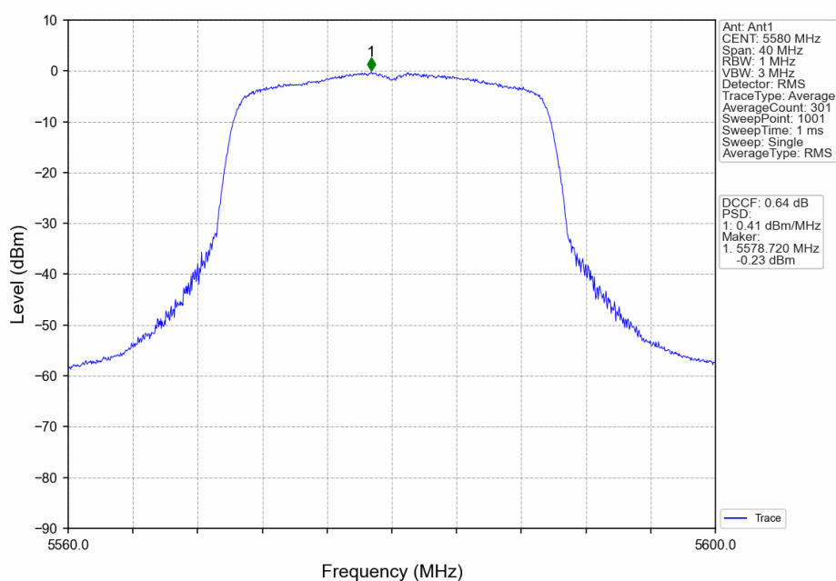
802.11ax(HEW20)_MCH_5580MHz_RU242_Left_Ant1_NTNV
