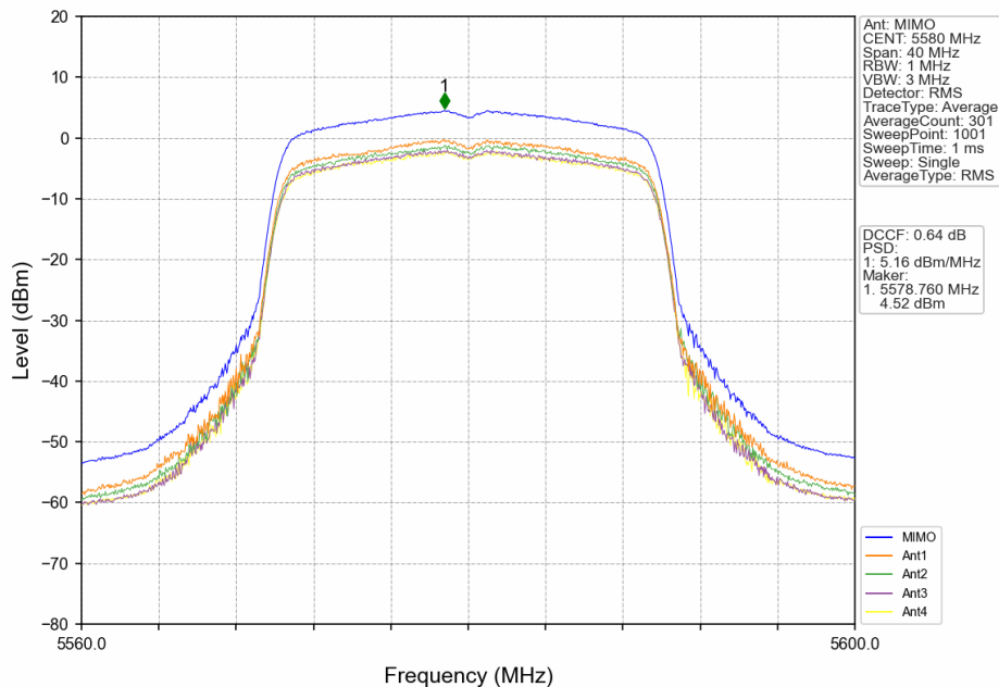
802.11ax(HEW20)_MCH_5580MHz_RU242_Left_MIMO_NTNV
