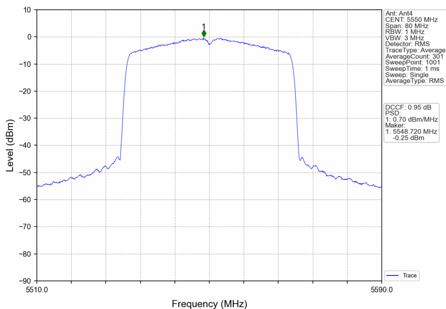
802.11ax(HEW40)_MCH_5550MHz_RU484_Left_Ant4_NTNV
