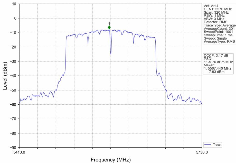
802.11ac(VHT160)_MCH_5570MHz_Ant4_NTNV
