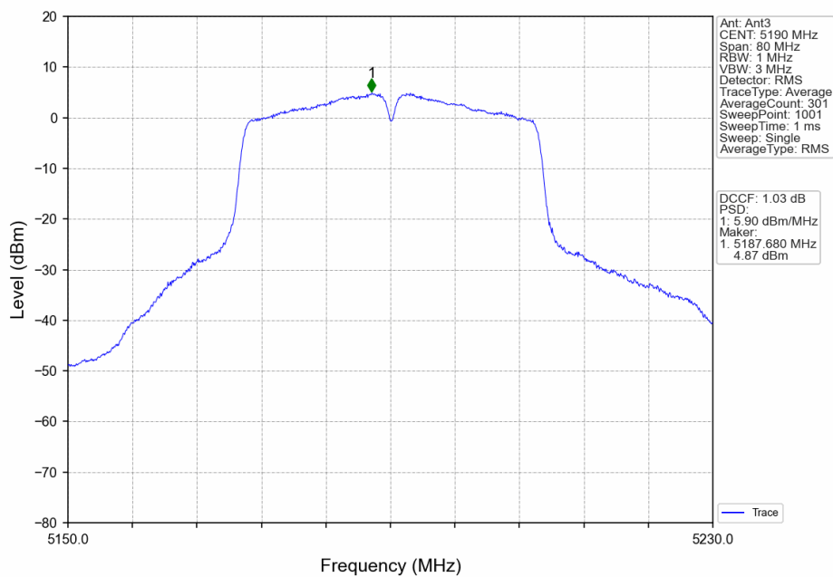
802.11ac(VHT40)_LCH_5190MHz_Ant3_NTNV
