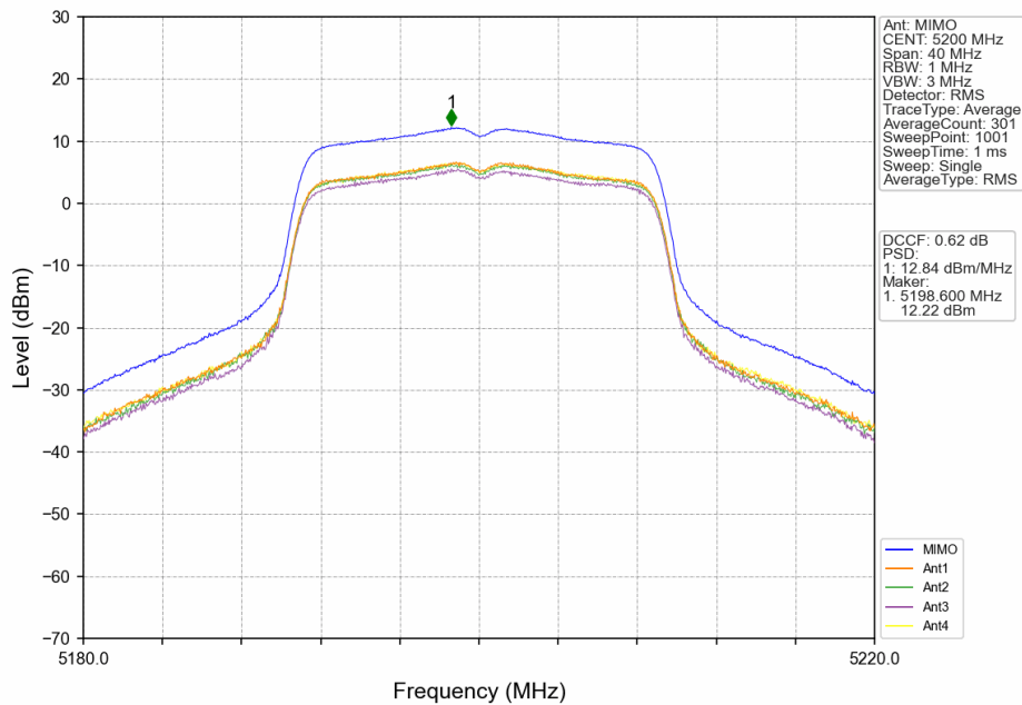
802.11ac(VHT20)_MCH_5200MHz_MIMO_NTNV
