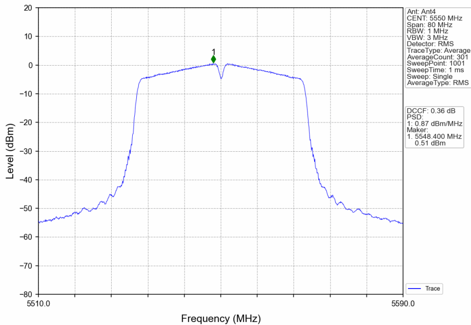
802.11n(HT40)_MCH_5550MHz_Ant4_NTNV
