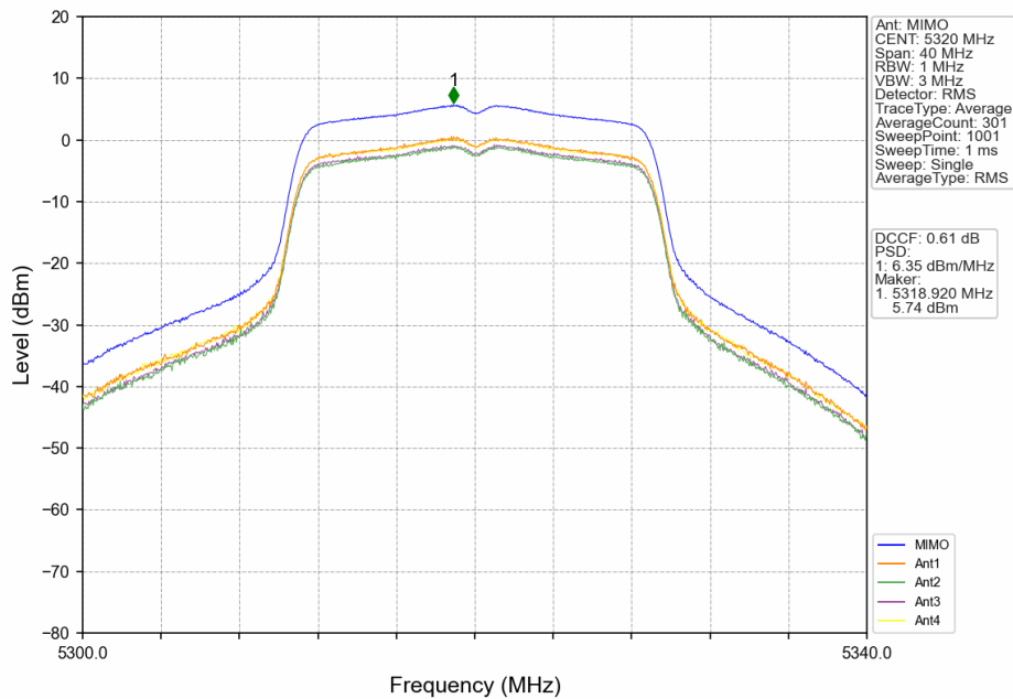
802.11ac(VHT20)_HCH_5320MHz_MIMO_NTNV
