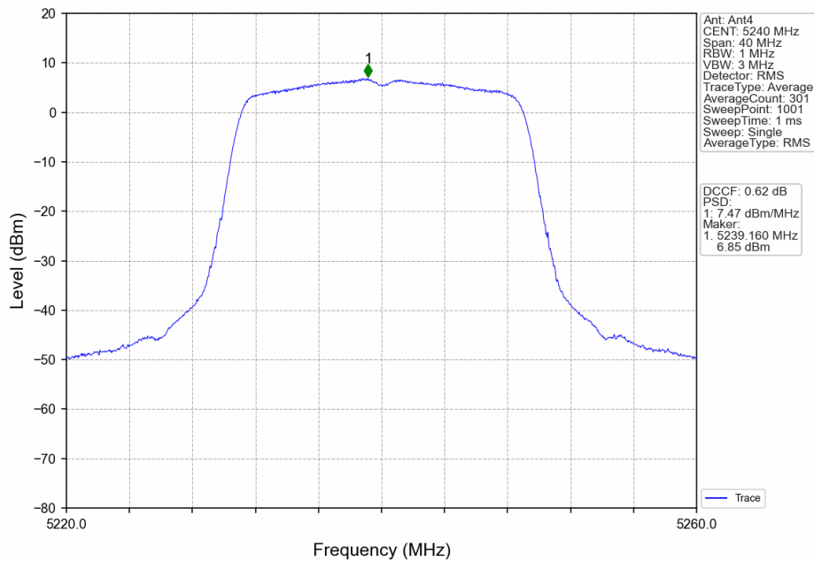
802.11ac(VHT20)_HCH_5240MHz_Ant4_NTNV
