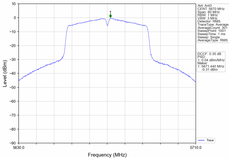
802.11n(HT40)_HCH_5670MHz_Ant3_NTNV
