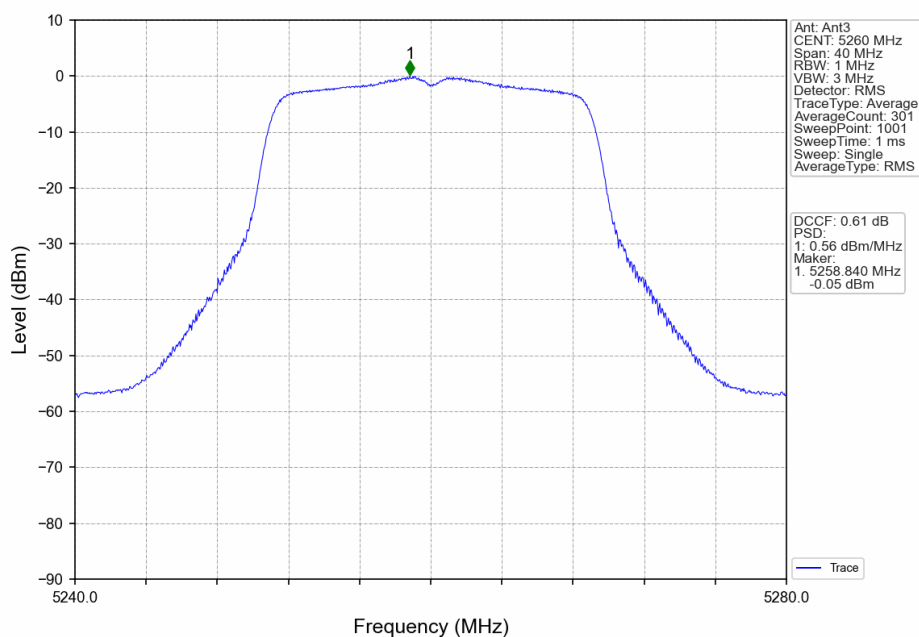
802.11ac(VHT20)_LCH_5260MHz_Ant3_NTNV
