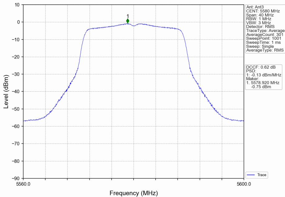
802.11ac(VHT20)_MCH_5580MHz_Ant3_NTNV
