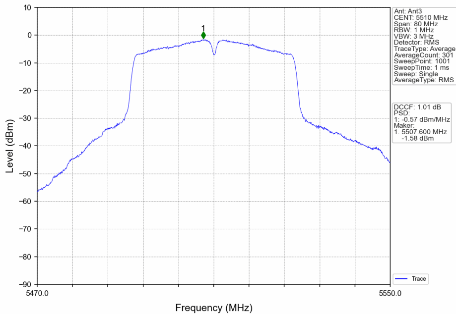
802.11ac(VHT40)_LCH_5510MHz_Ant3_NTNV
