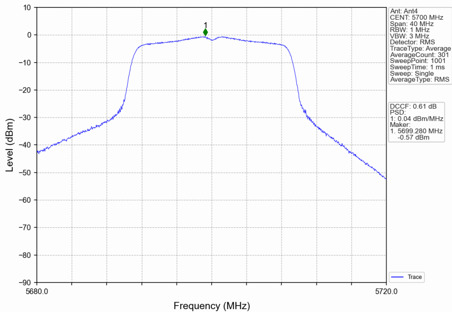
802.11ac(VHT20)_HCH_5700MHz_Ant4_NTNV
