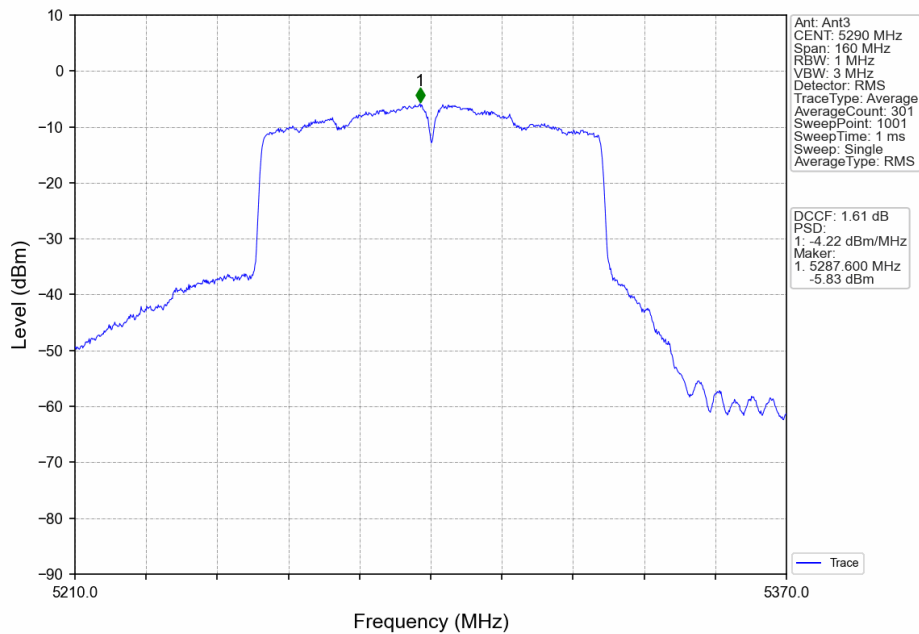
802.11ac(VHT80)_MCH_5290MHz_Ant3_NTNV
