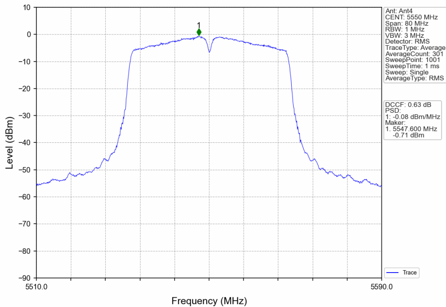
802.11ac(VHT40)_MCH_5550MHz_Ant4_NTNV
