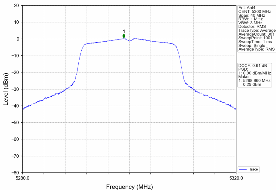
802.11ac(VHT20)_MCH_5300MHz_Ant4_NTNV
