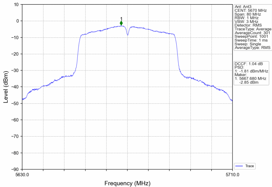
802.11ac(VHT40)_HCH_5670MHz_Ant3_NTNV
