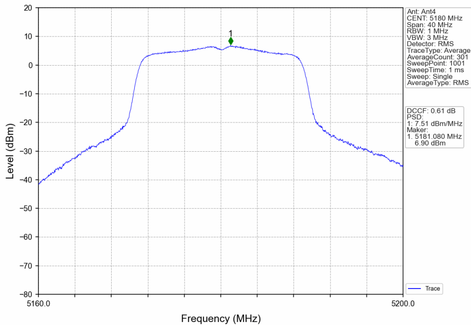
802.11ac(VHT20)_LCH_5180MHz_Ant4_NTNV
