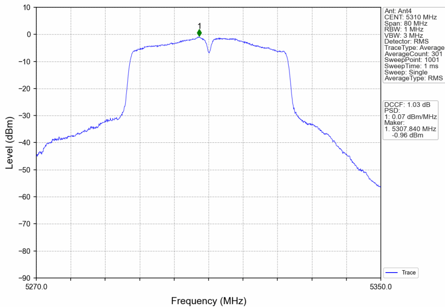
802.11ac(VHT40)_HCH_5310MHz_Ant4_NTNV
