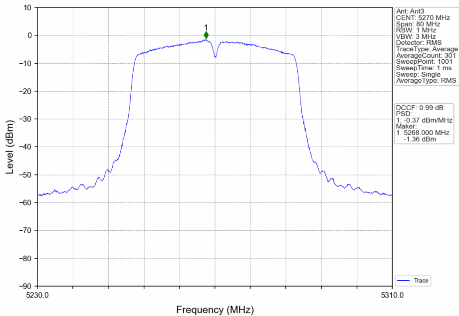
802.11ac(VHT40)_LCH_5270MHz_Ant3_NTNV
