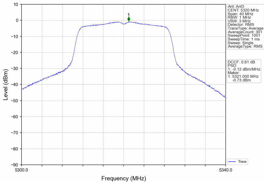
802.11ac(VHT20)_HCH_5320MHz_Ant3_NTNV
