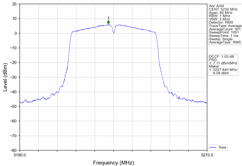
802.11ac(VHT40)_HCH_5230MHz_Ant4_NTNV
