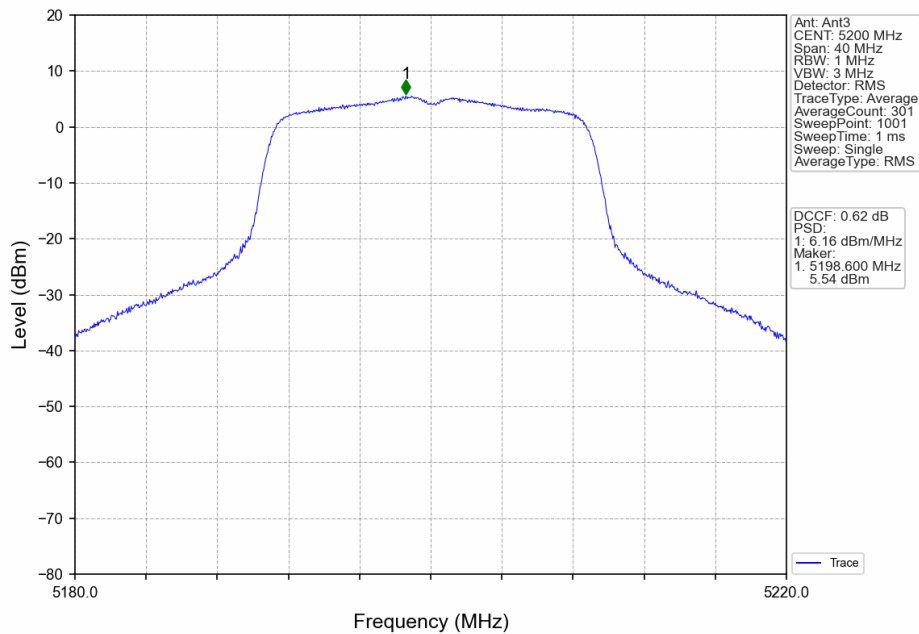
802.11ac(VHT20)_MCH_5200MHz_Ant3_NTNV
