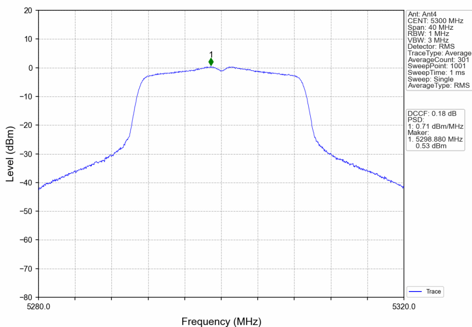
802.11n(HT20)_MCH_5300MHz_Ant4_NTNV
