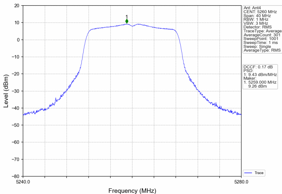
802.11a_LCH_5260MHz_Ant4_NTNV
