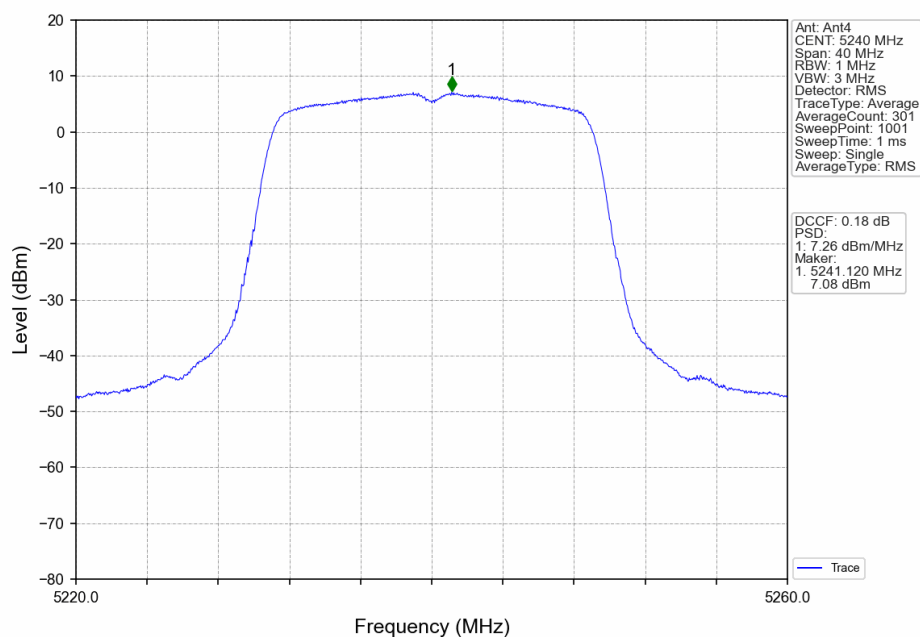
802.11n(HT20)_HCH_5240MHz_Ant4_NTNV
