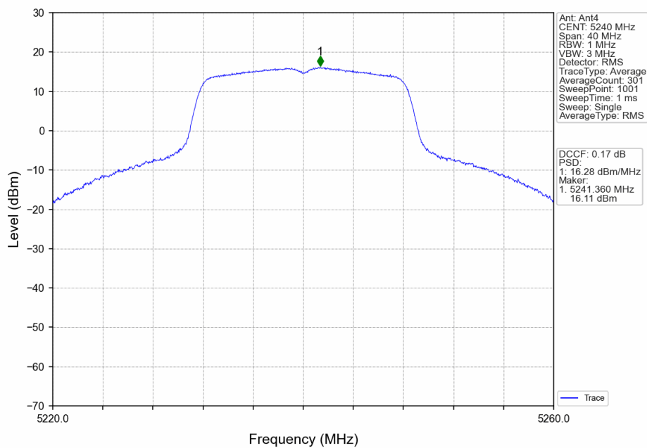
802.11a_HCH_5240MHz_Ant4_NTNV
