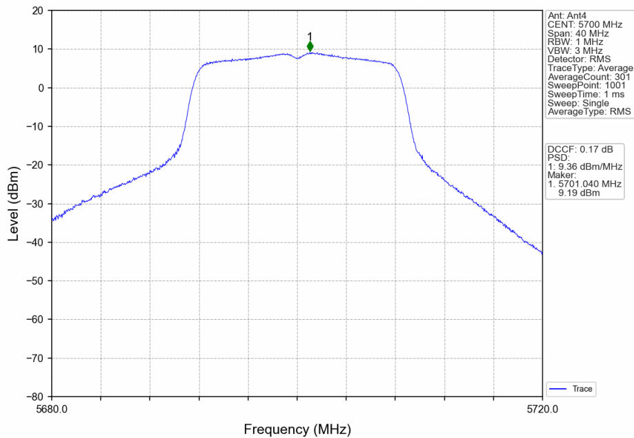
802.11a_HCH_5700MHz_Ant4_NTNV
