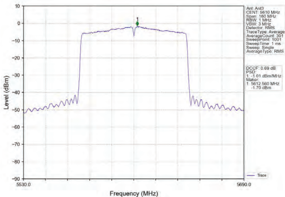
802.11ac(VHT80)_HCH_5610MHz_Ant3_NTNV
