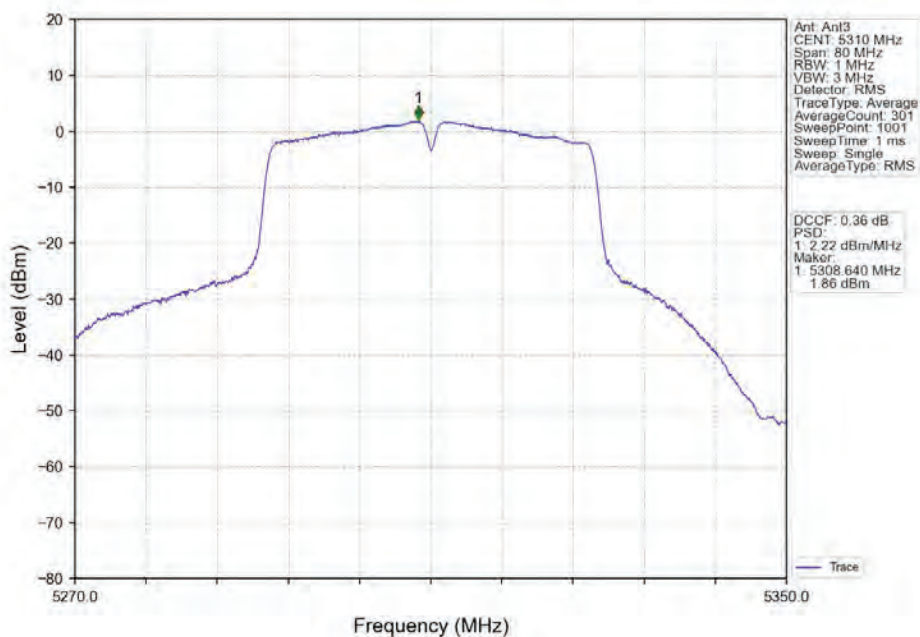
802.11ac(VHT40)_HCH_5310MHz_Ant3_NTNV
