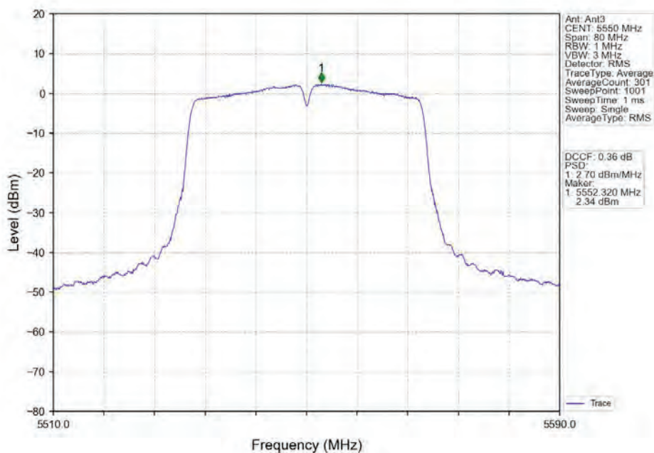
802.11ac(VHT40)_MCH_5550MHz_Ant3_NTNV
