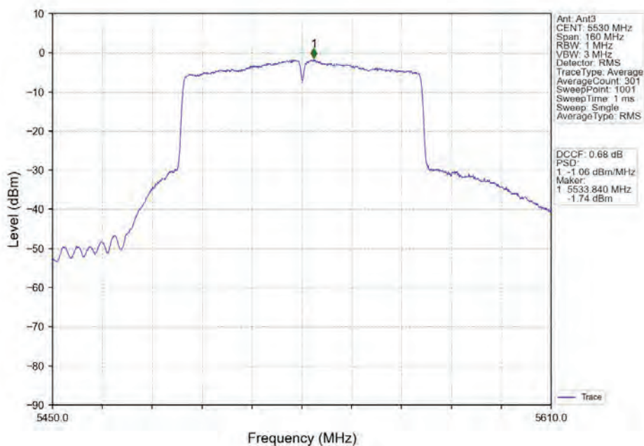
802.11ac(VHT80)_LCH_5530MHz_Ant3_NTNV
