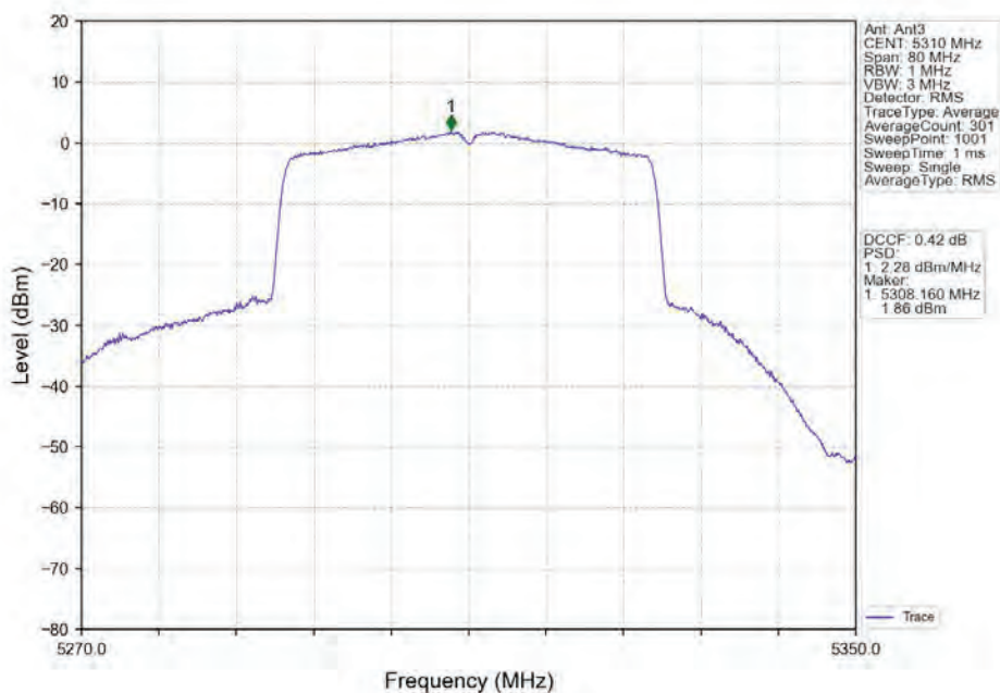
802.11ax(HEW40)_HCH_5310MHz_RU484_Left_Ant3_NTNV
