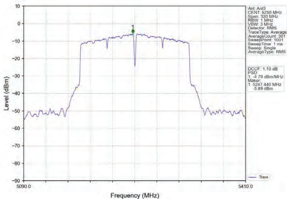
802.11ac(VHT160)_MCH_5250MHz_Ant3_NTNV
