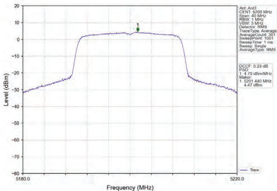
802.11ax(HEW20)_MCH_5200MHz_RU242_Left_Ant3_NTNV
