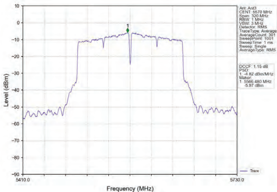
802.11ac(VHT160)_MCH_5570MHz_Ant3_NTNV
