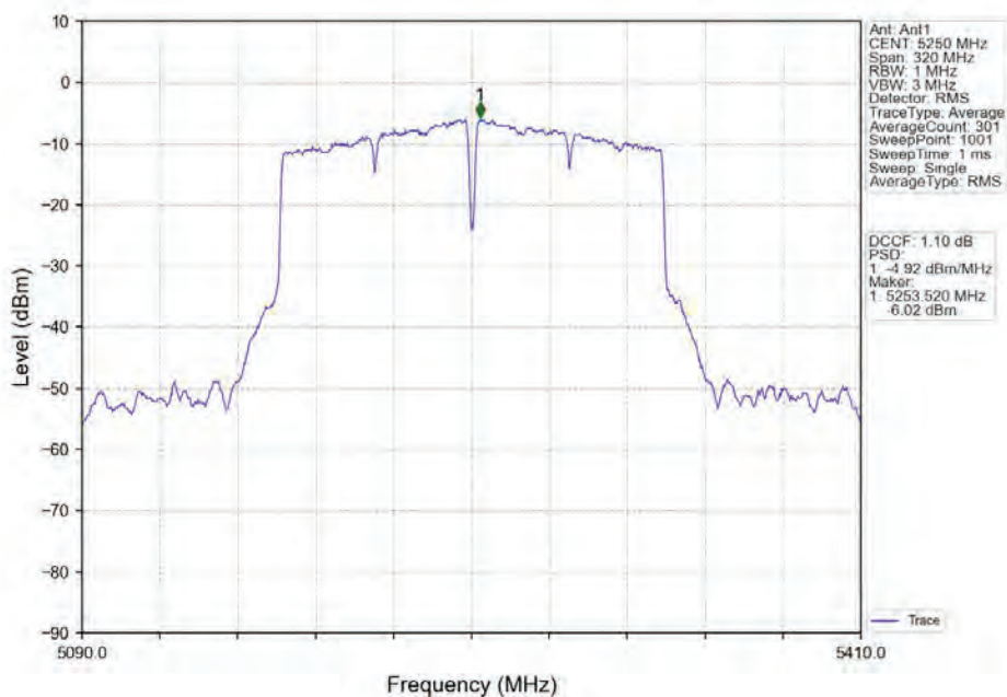
802.11ac(VHT160)_MCH_5250MHz_Ant1_NTNV
