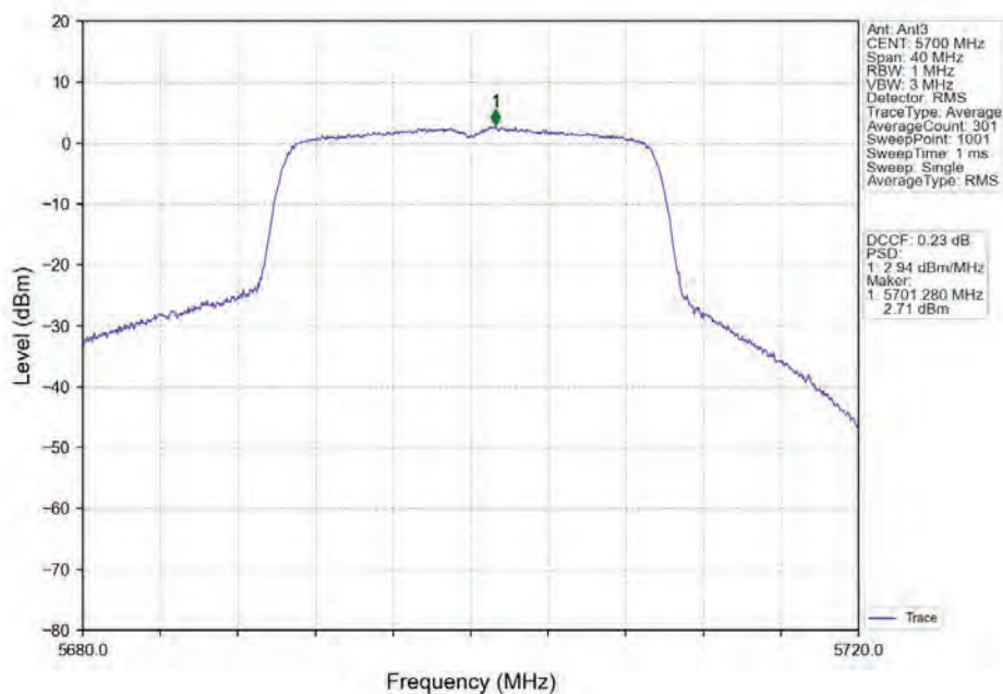
802.11ax(HEW20)_HCH_5700MHz_RU242_Left_Ant3_NTNV
