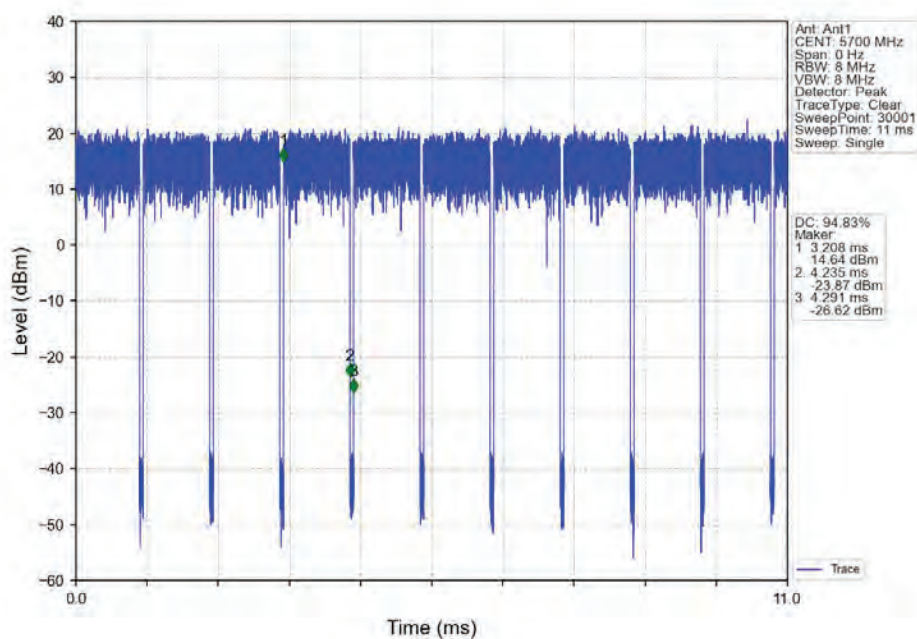
802.11ax(HEW20)_HCH_5700MHz_RU242_Left_Ant1_NTNV
