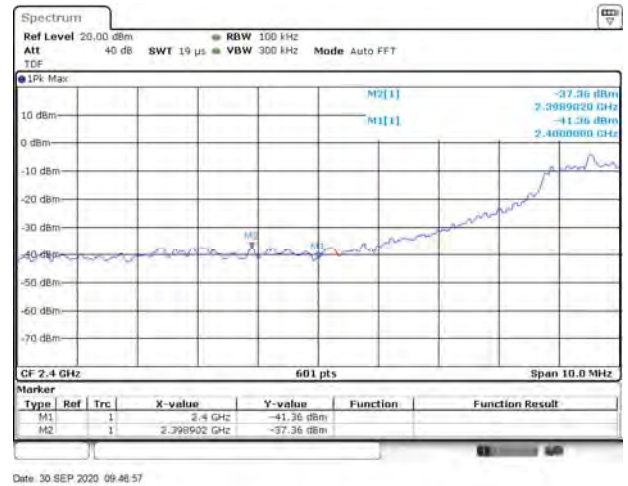
802.11n-40 MHz LOW CHANNEL, Reference level
