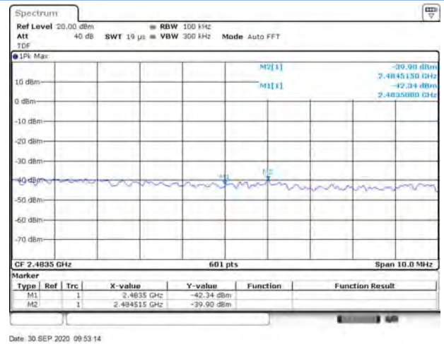
802.11n-40 MHz HIGH CHANNEL, Reference level
