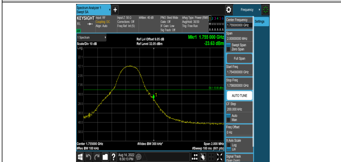
Band4-5MHz-16QAM-20375-1RB#24
